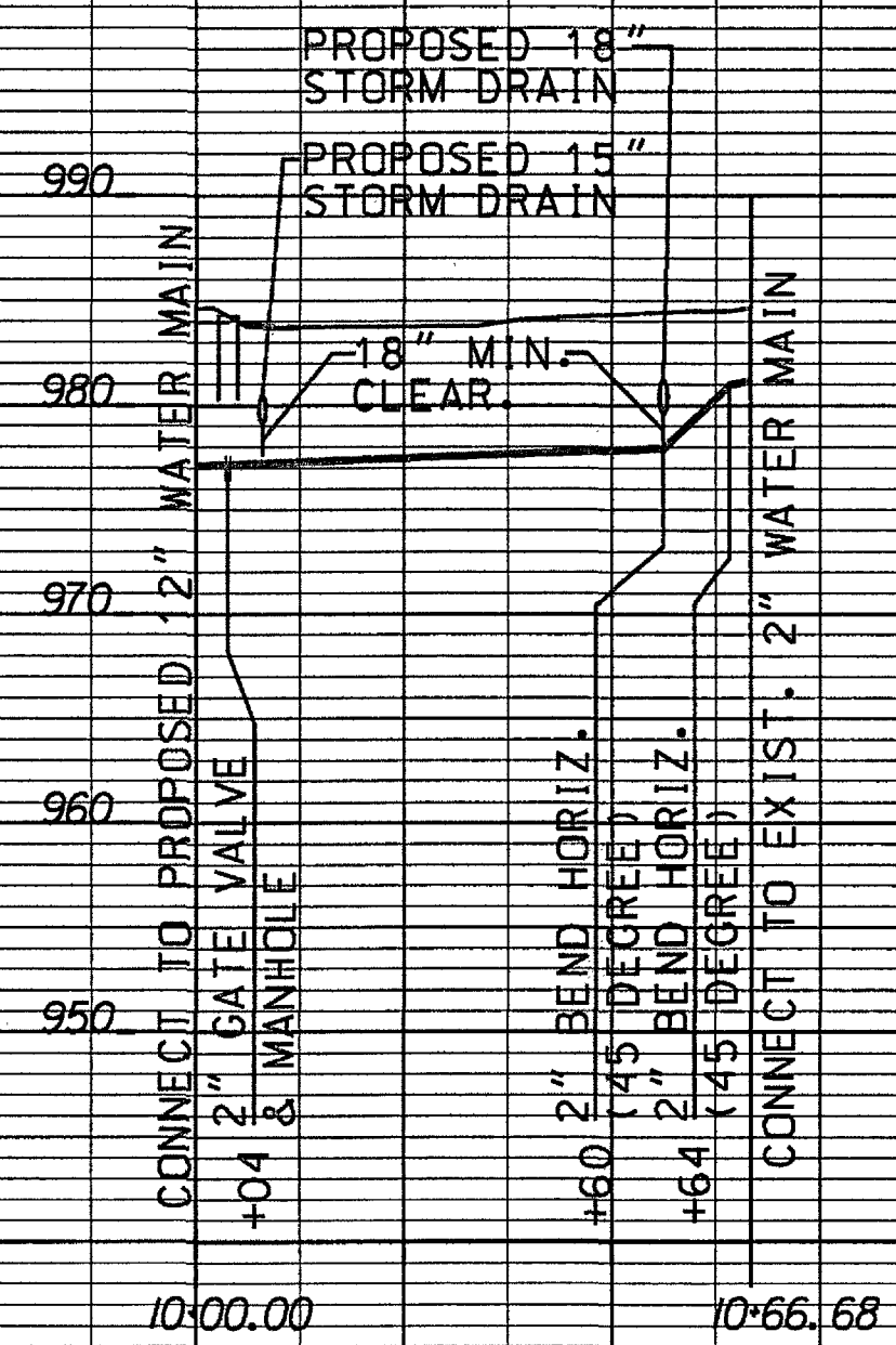
2" WATER MAIN, PLAN SHEET 23(7) APPROX. STA. 132+95.19' RT. CONST. B ON 10TH STREET TO APPROX. STA. 10+83.11' LT. CONST. B ON GRAYSON AVE (EAST)
