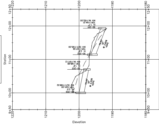
Storm 2 PROFILE
