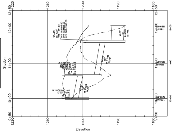
Storm 1 PROFILE
