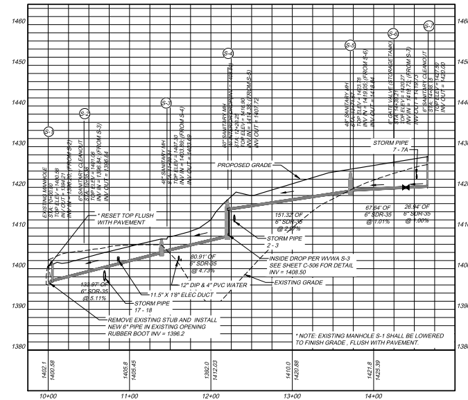
WATER LINE PROFILE
