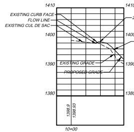
SWM POND SERVICE ENTRANCE PROFILE
