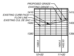
MAIN ENTRANCE PROFILE CG-13
