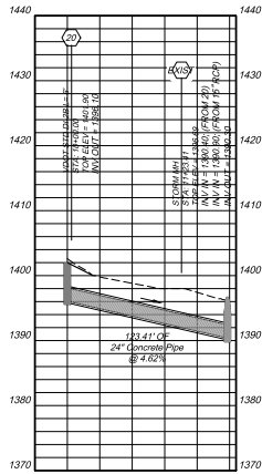
STRUCTURE 20 TO EXISTING MH PROFILE
