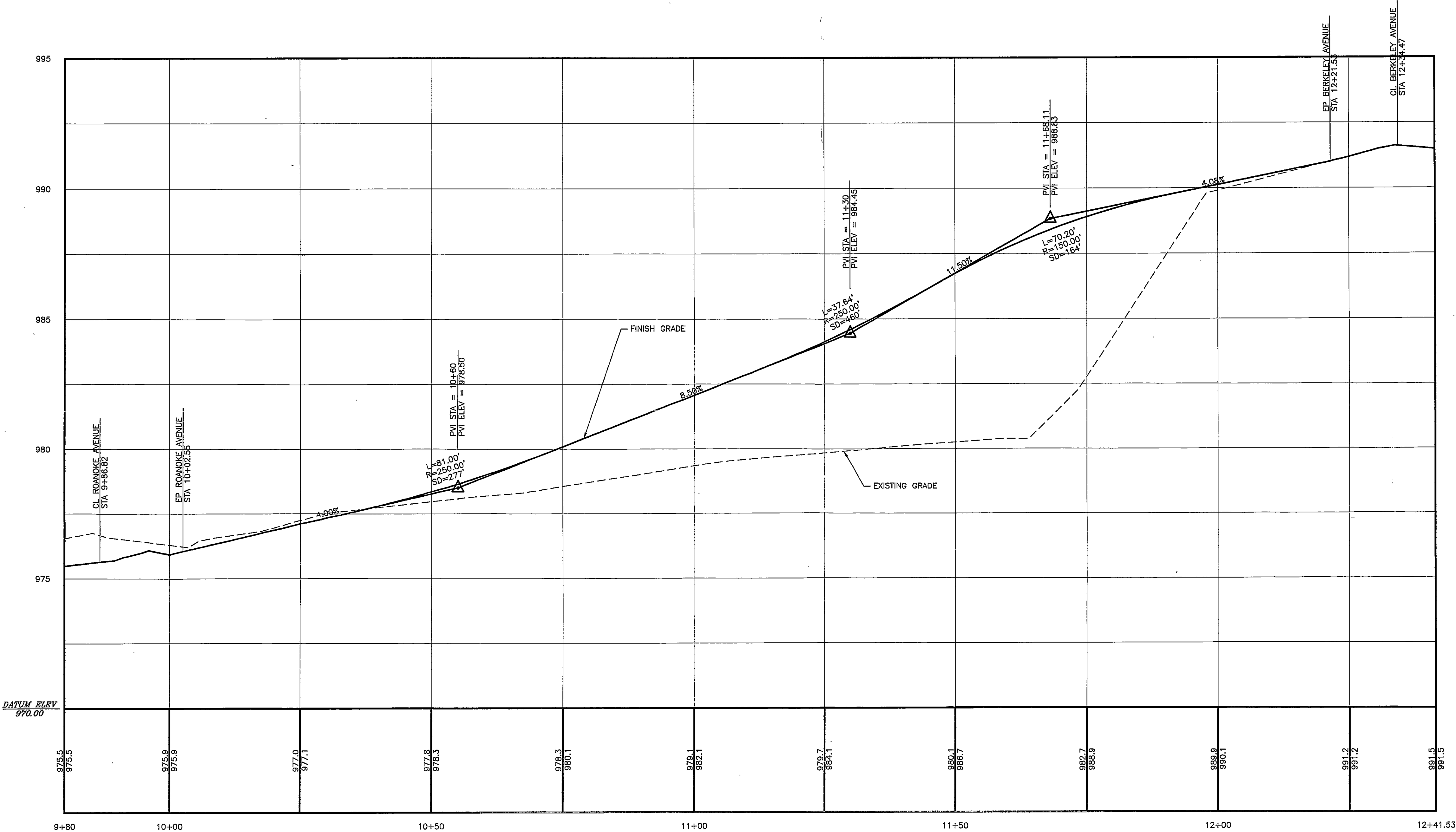
ROANOKE AVENUE REALIGNMENT PROFILE
