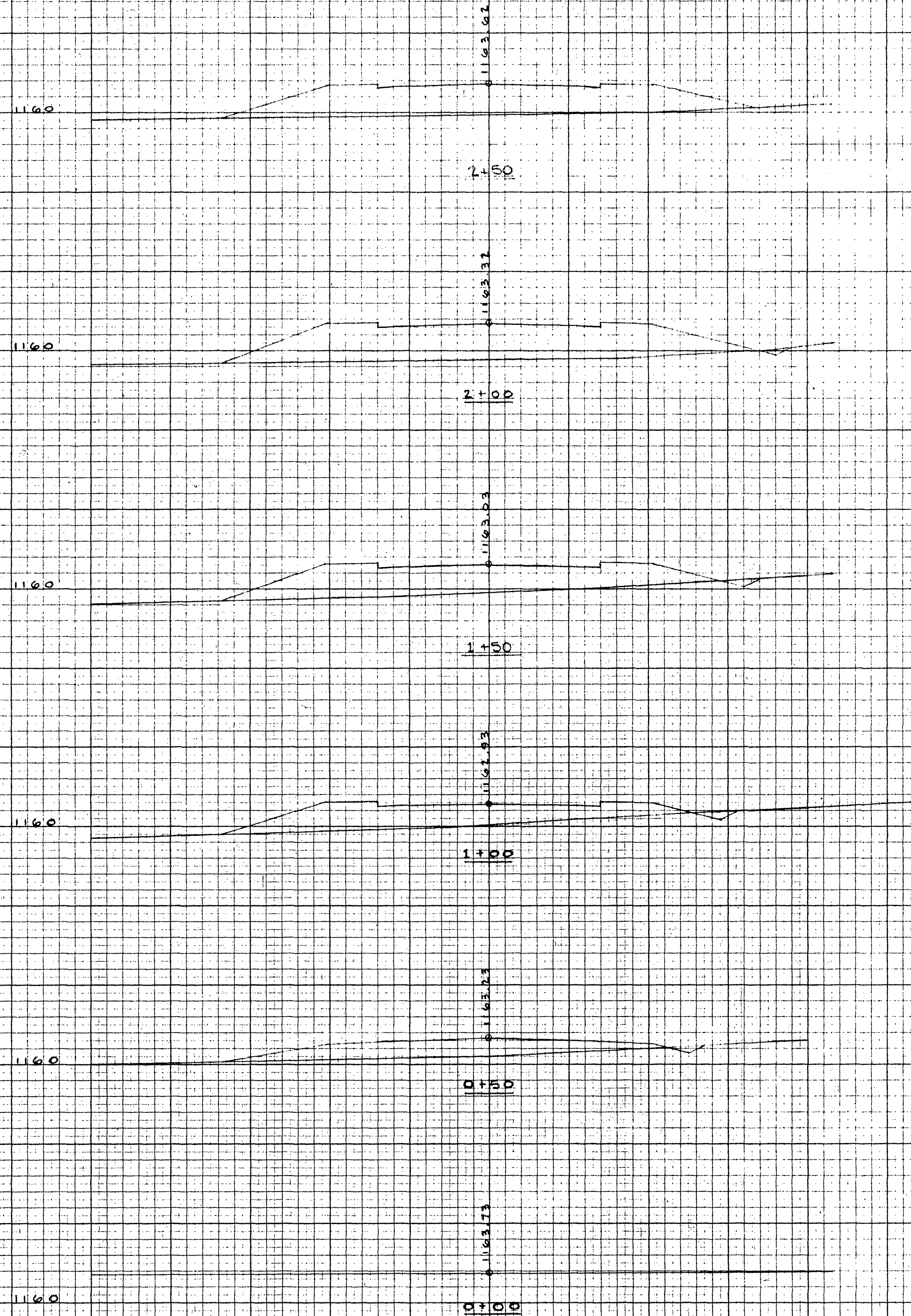
ACCESS ROAD CROSS SECTIONS SCALE: 1" = 10'-0" VERTICAL 1" = 10'-0" HORIZONTAL
