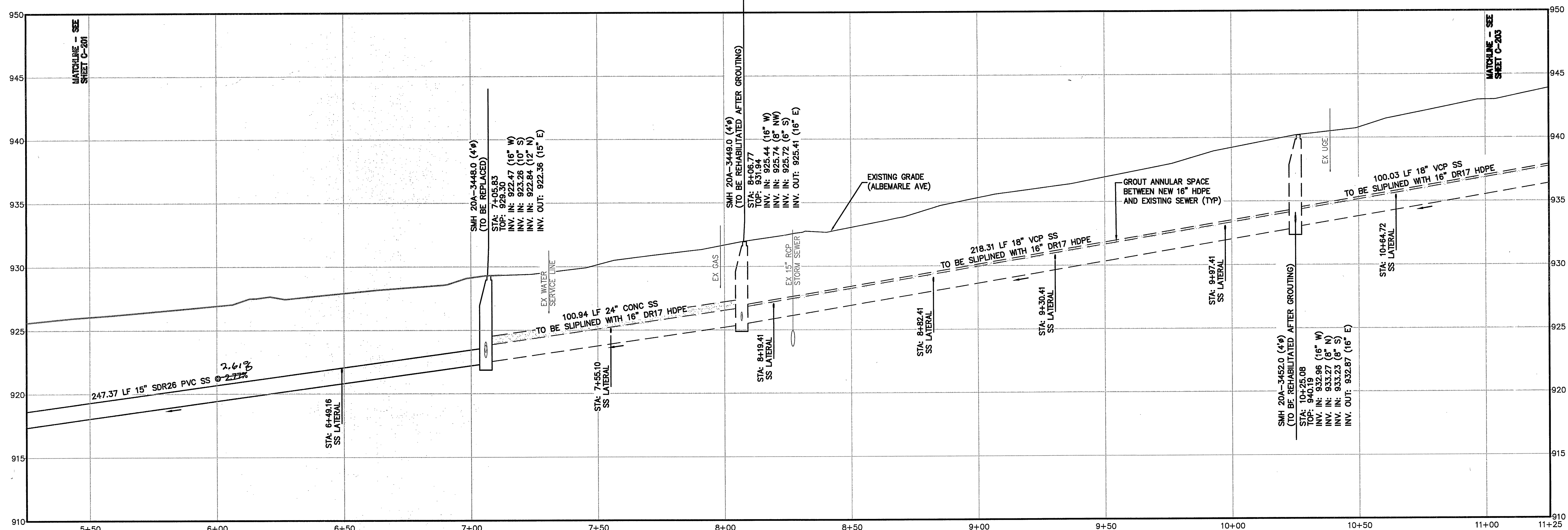
SEWER PROFILE SCALE: H: 1"=20', V: 1"=4'
