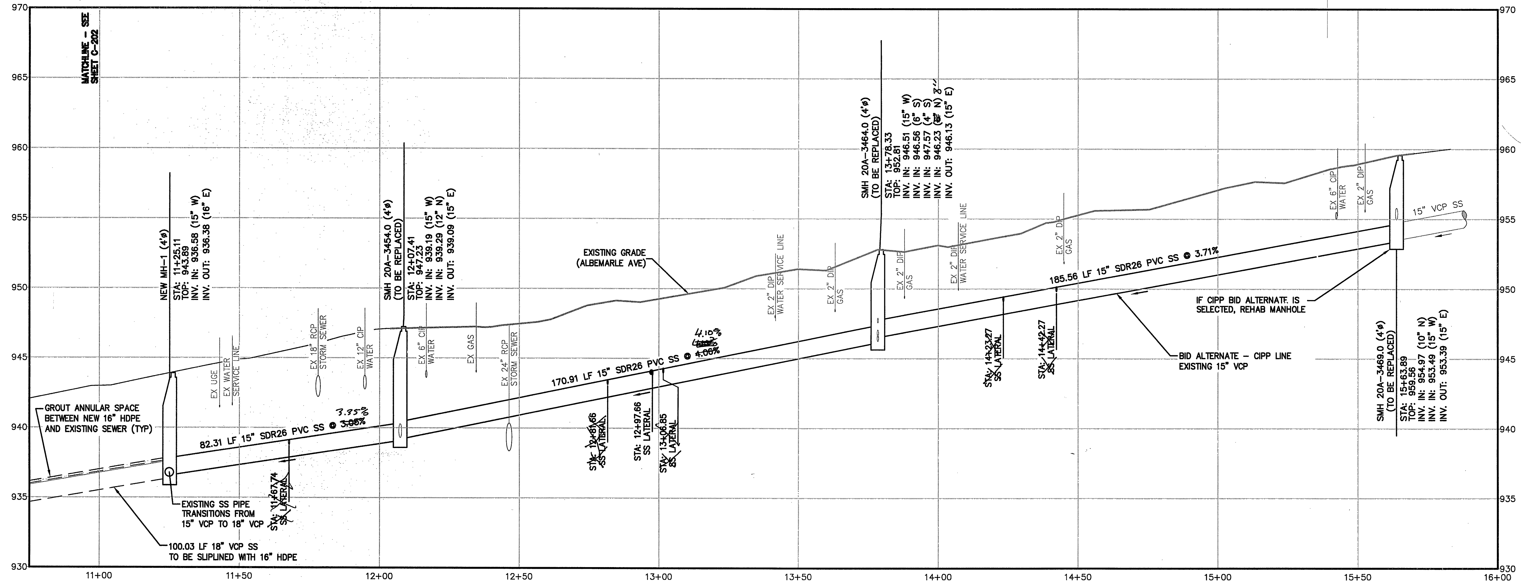
SEWER PROFILE SCALE: H: 1"=20', V: 1"=4'
