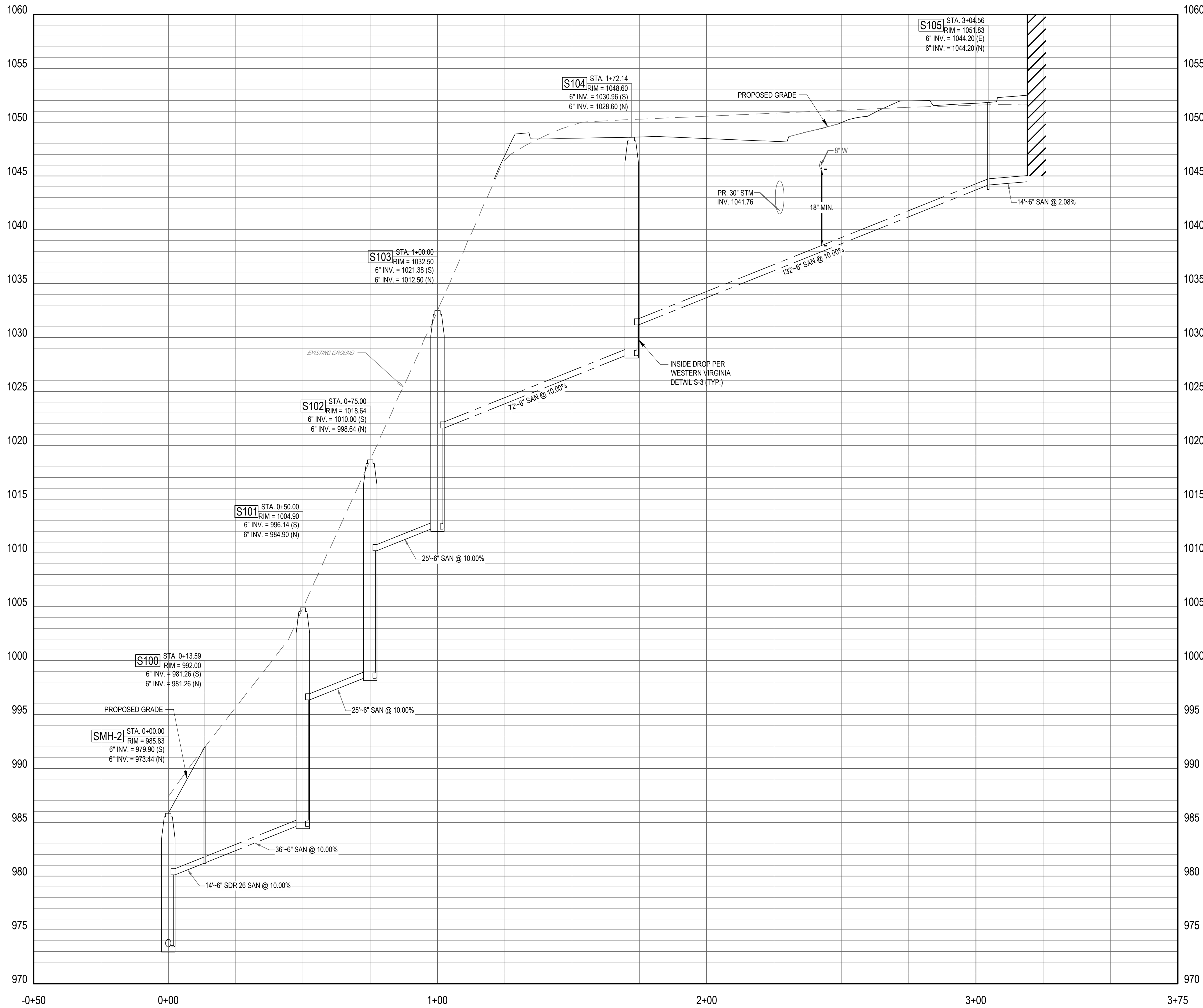
SANITARY PROFILE SCALE: 1" = 20' HORIZ.; 1" = 5' VERT.
