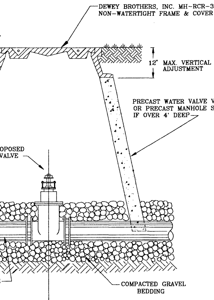
WATER LINE VALVE INSTALLATION
