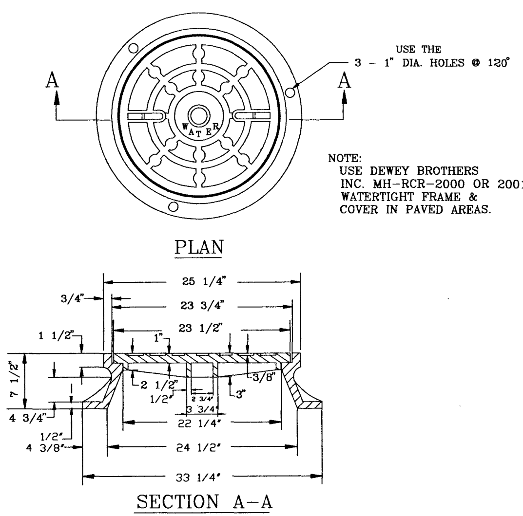
MANHOLE FRAME AND COVER PAVED 2001EC UNPAVED 2001(ABOVE)
