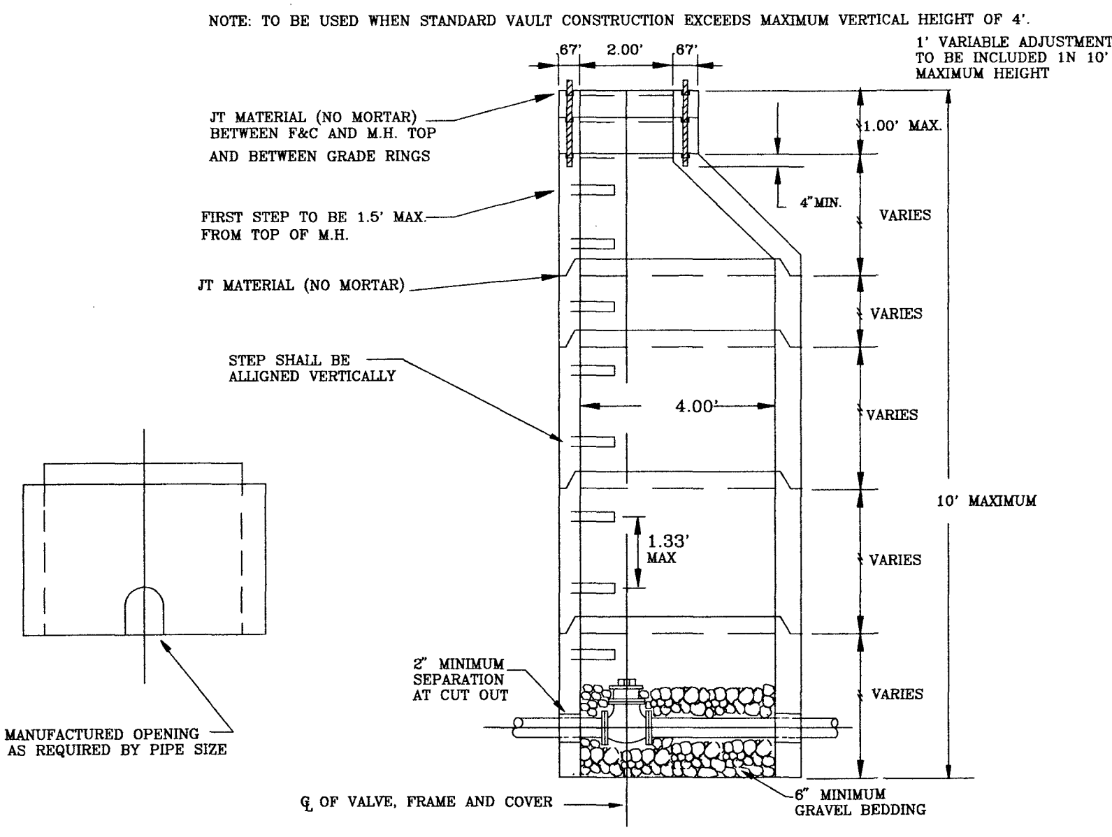
ALTERNATE VALVE VAULT (MANHOLE)
