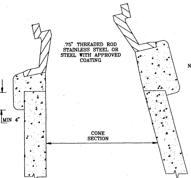
INSTALLATION DETAIL FOR ALL FRAMES AND COVERS
