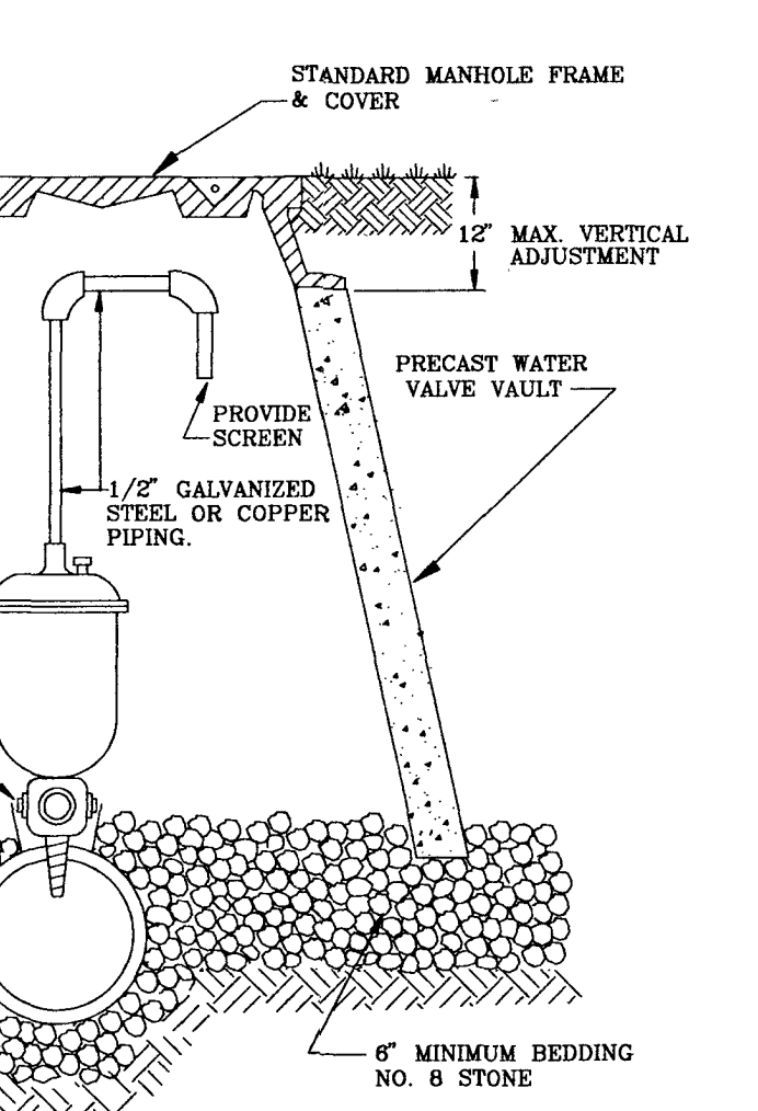
AUTOMATIC AIR RELEASE ASSEMBLY
