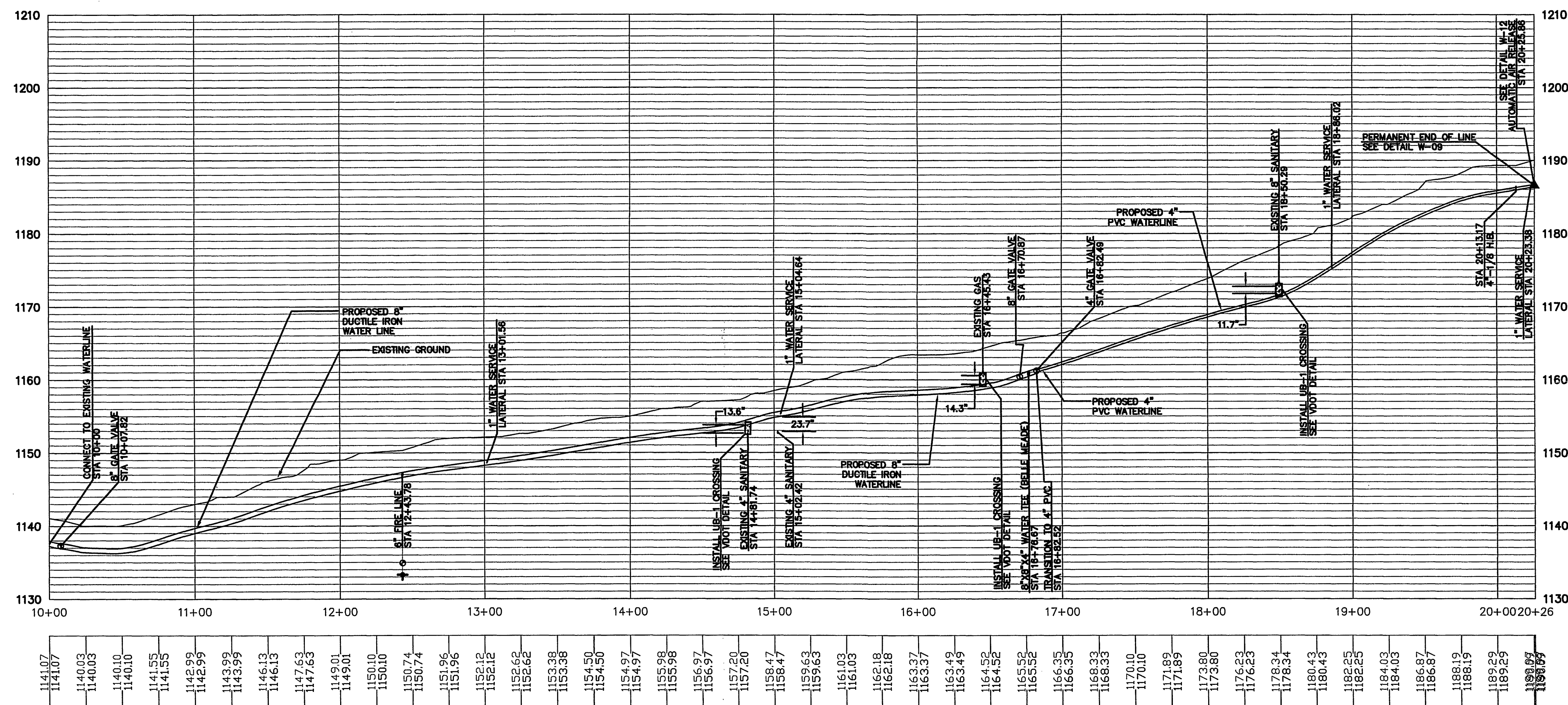
TOPPING HILL DR. SEC. PROFILE SCALE: 1"=50'H, 1"=10'V
