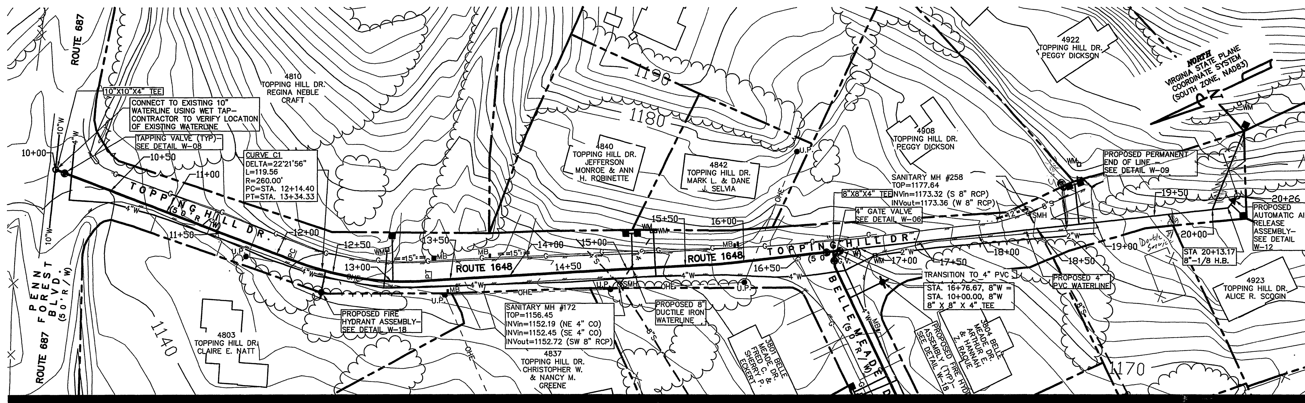
TOPPING HILL DR. SEC. PLAN SCALE: 1"=50'
