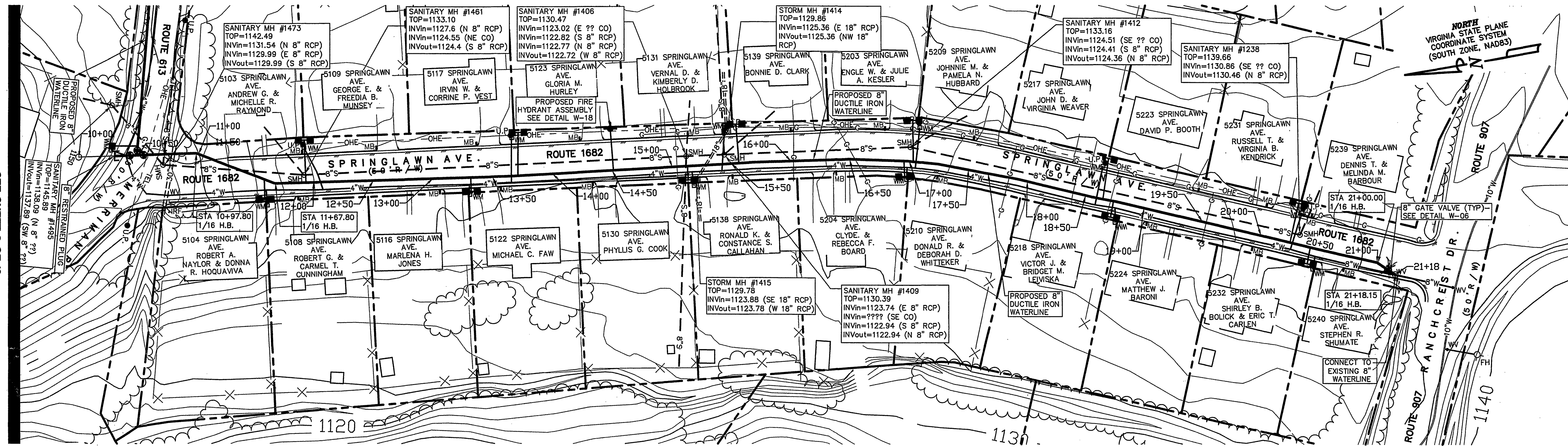
SPRINGLAWN AVE. SEC. PLAN SCALE: 1"=50'
