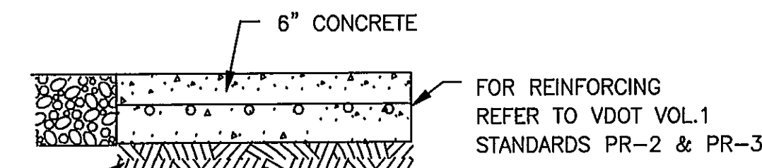
SECTION THROUGH DUMPSTER PAD NO SCALE
