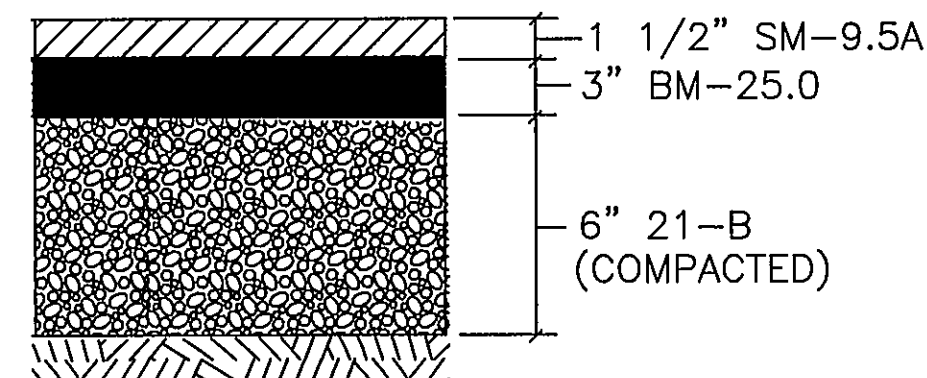
ROUTE 117 PAVEMENT SECTION NO SCALE NOTE: MATCH MAINLINE PAVEMENT STRUCTURE IF GREATER
