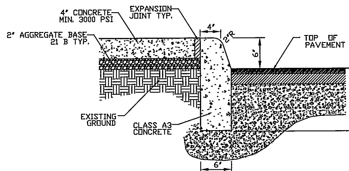
TYPICAL SIDEWALK DETAIL NO SCALE
