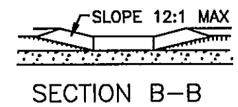
H.C. CURB RAMP NO SCALE
