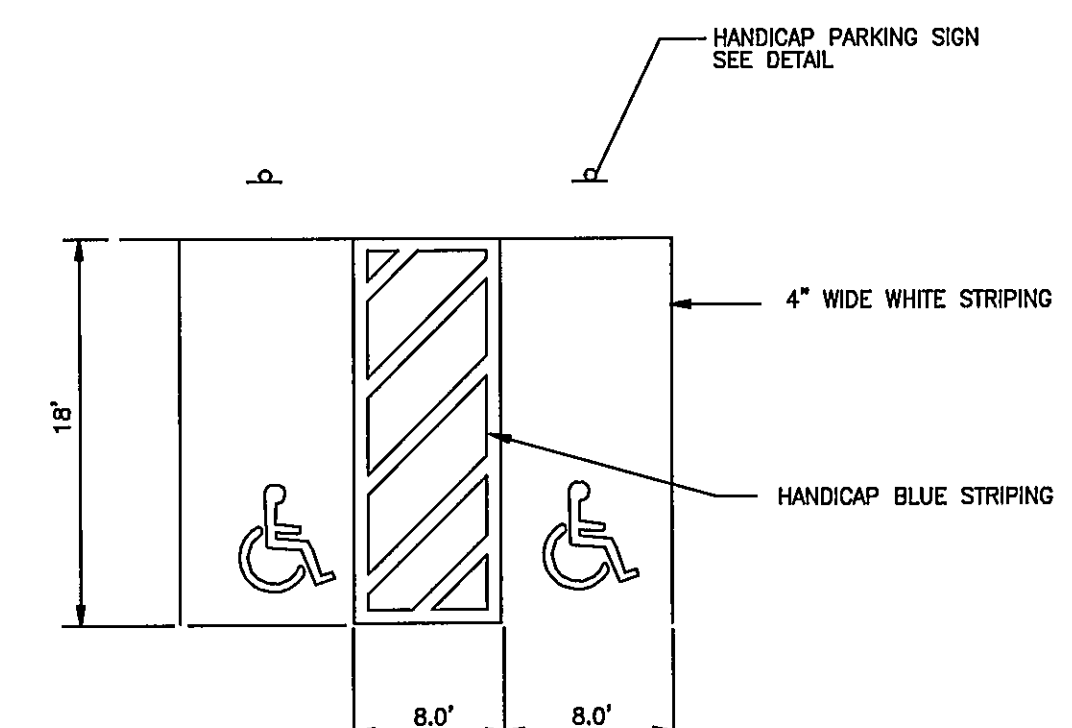
HANDICAPPED PARKING DETAIL N.T.S.
