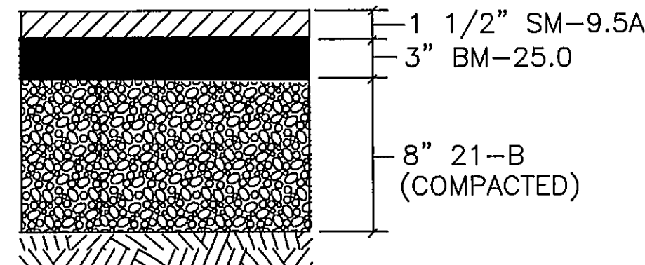
HEAVY DUTY/ROADWAY PAVEMENT SECTION NO SCALE
