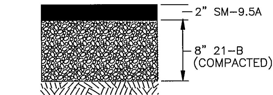
STD PAVEMENT SECTION NO SCALE
