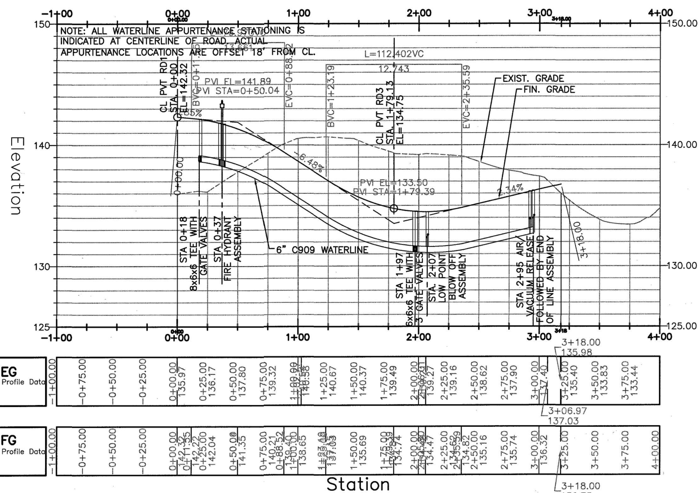
PROFILE - PVT RD 2 SUNRISE LANE (PRIVATE)
