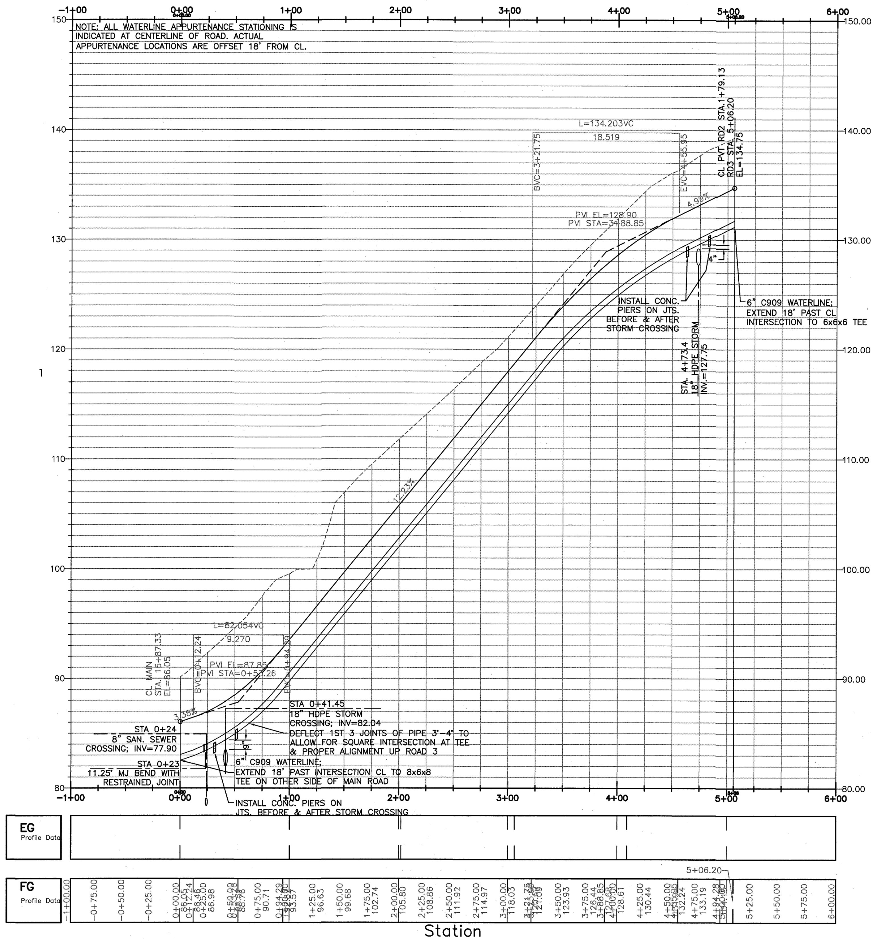
PROFILE - PVT RD 3 CARRINGTON COURT (PRIVATE)
