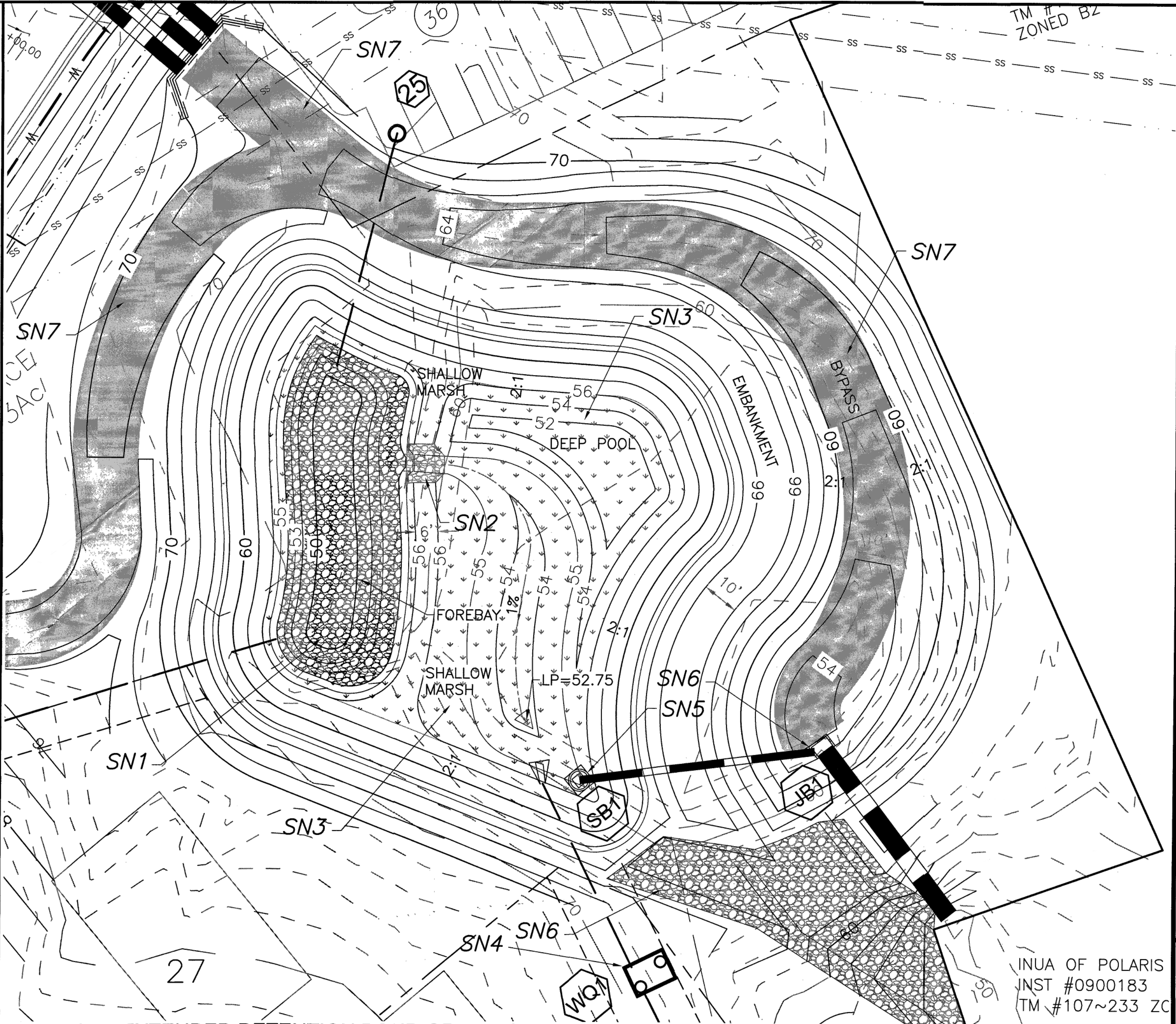
ENHANCED EXTENDED DETENTION POND GRADING SCALE: 1"=20'
