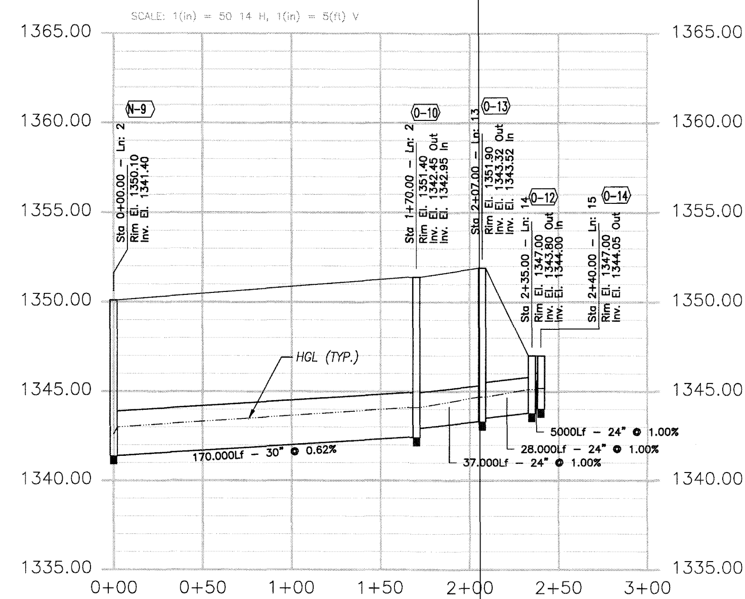
(STR EX. N-9 - O-14) STORM DRAIN PROFILE
