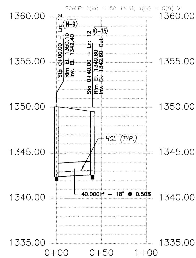
(STR EX. N-9 - O-15) STORM DRAIN PROFILE
