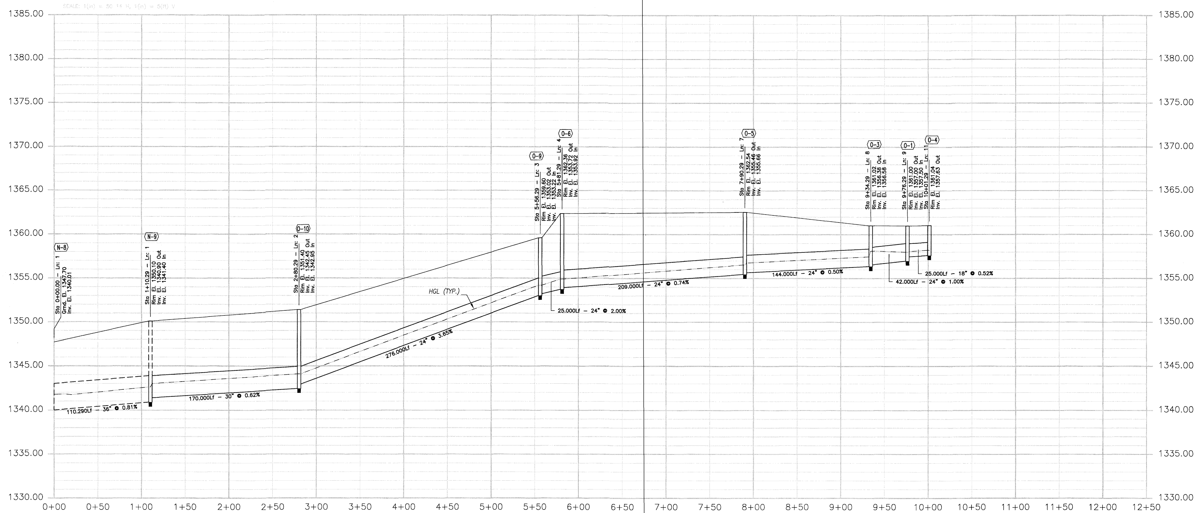
(STR EX. N-8 - O-4) STORM DRAIN PROFILE
