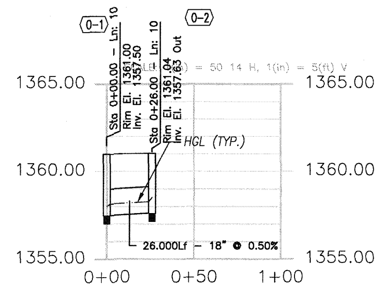
(STR EX. O-1 - O-2) STORM DRAIN PROFILE
