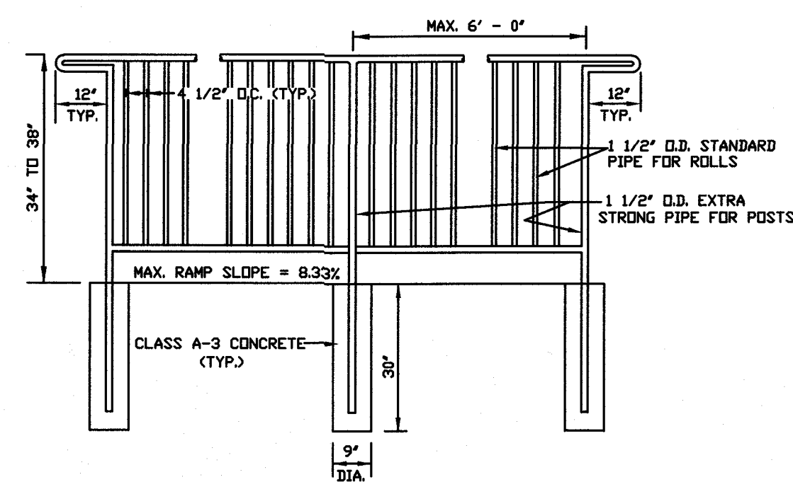
HANDRAIL DETAIL
