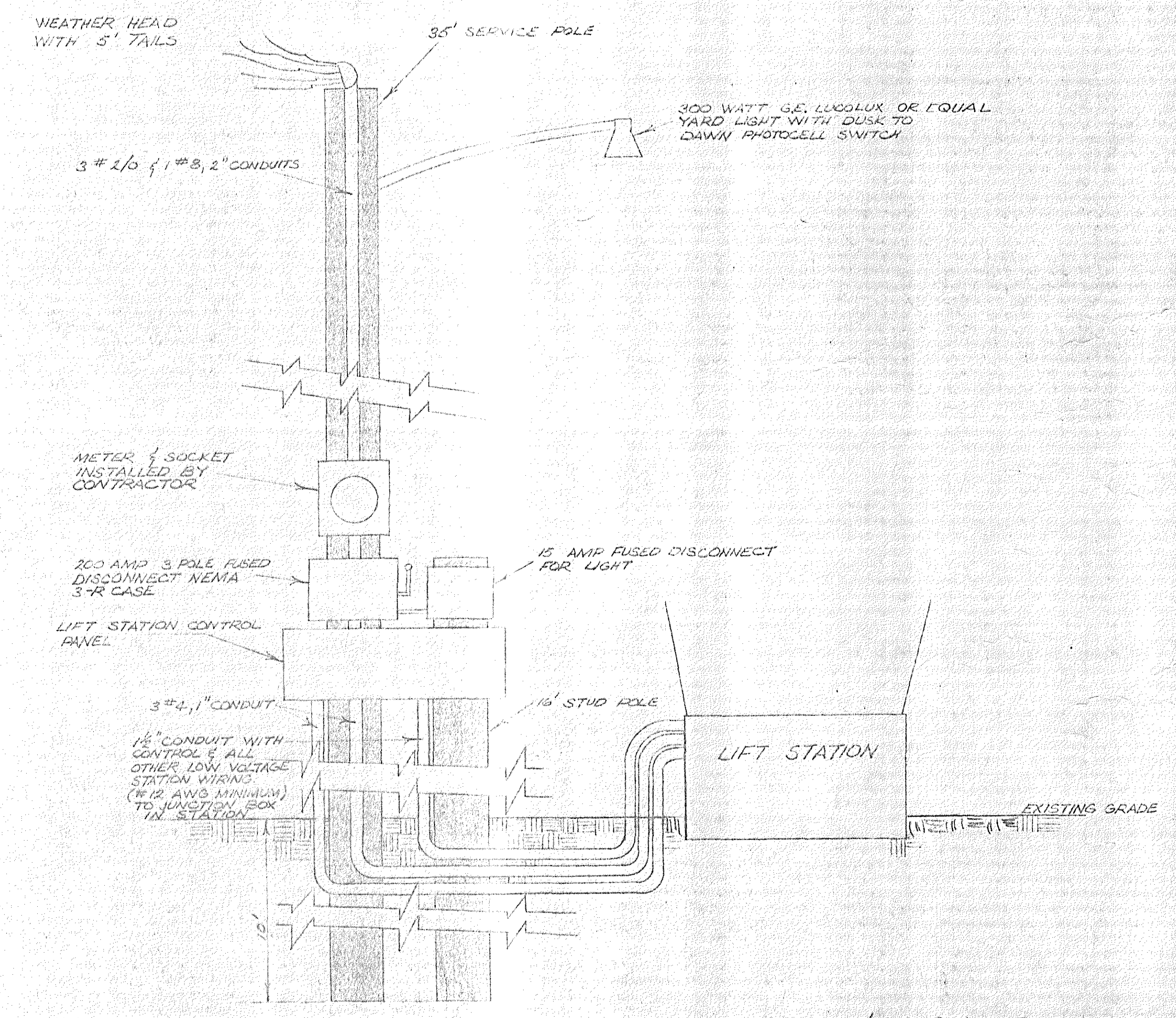
TYPICAL SERVICE POLE & YARD LIGHT NO SCALE
