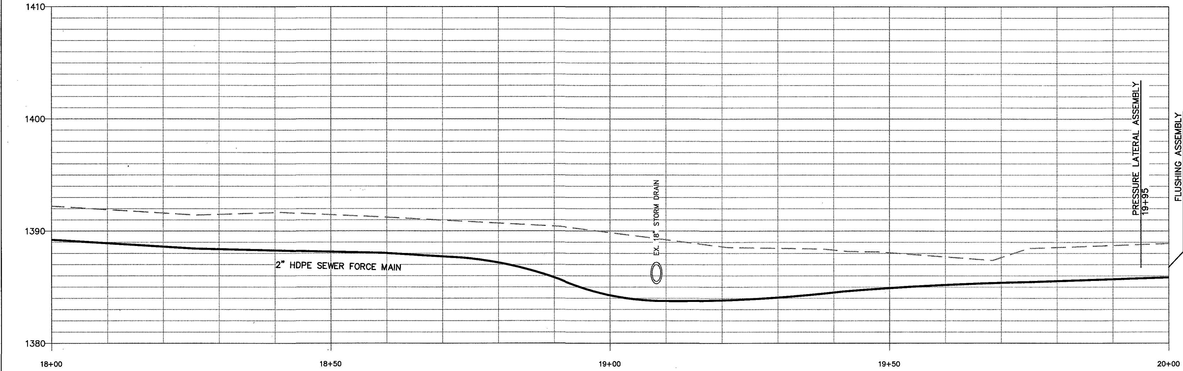
SEWER FORCEMAIN "A" SCALE VERTICAL: 1" = 5' HORIZONTAL: 1" = 10'
