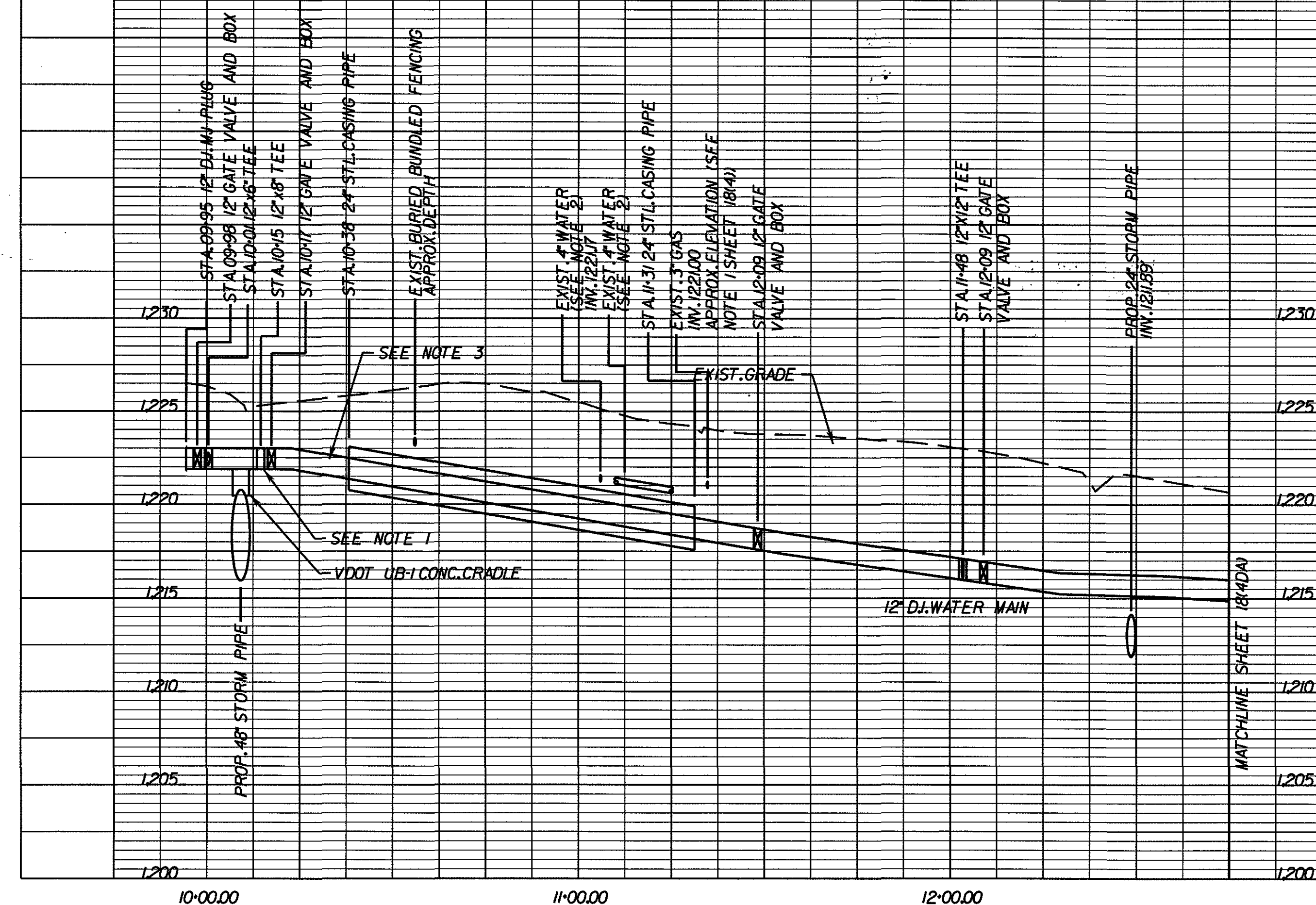
WATER MAIN "B" PROFILE
