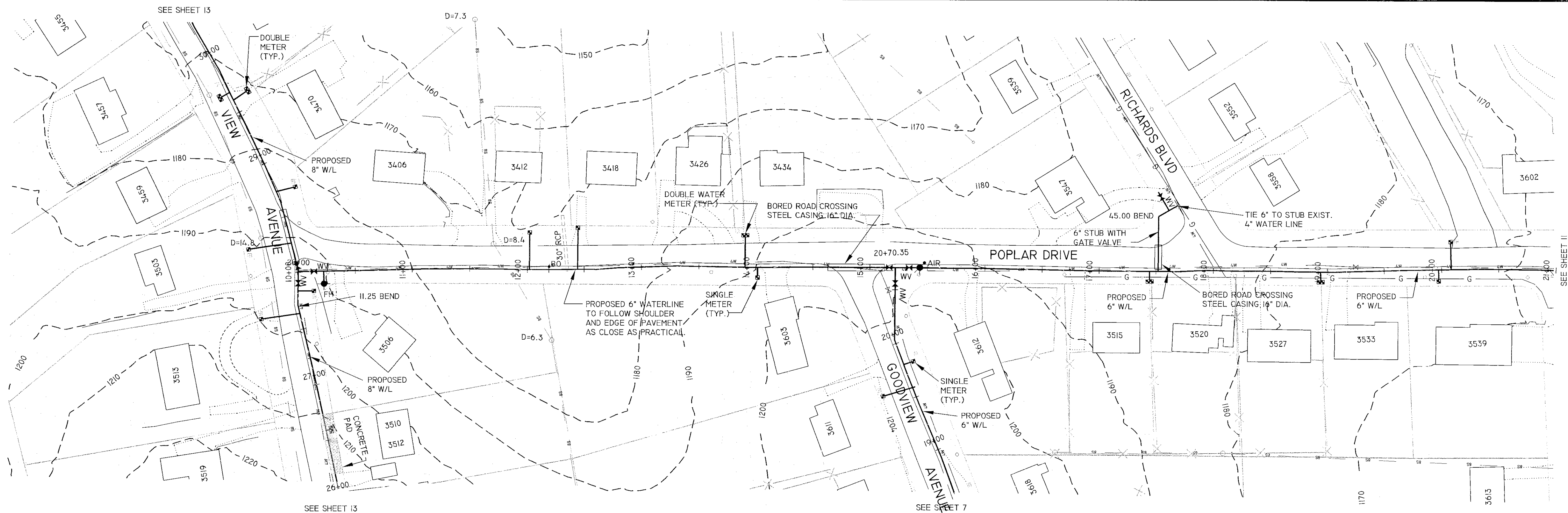
PLAN SCALE: 1"=50'
