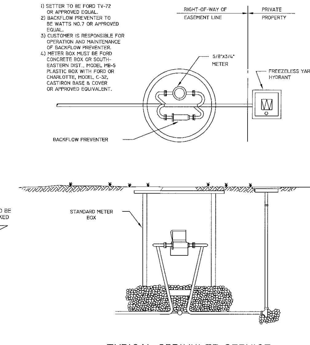
TYPICAL SPRINKLER SERVICE
