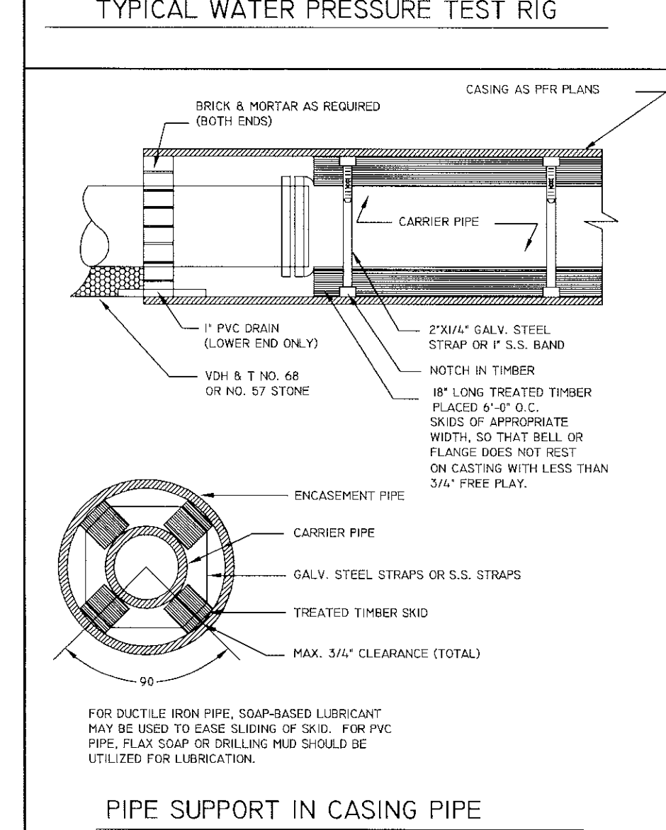
PIPE SUPPORT IN CASING PIPE
