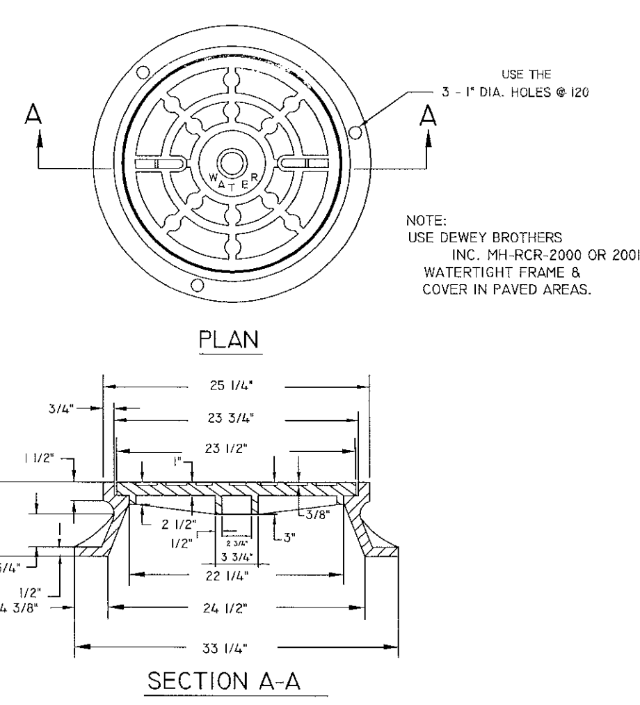
MANHOLE FRAME AND COVER PAVED 2001C UNPAVED 2001(A)BOVE
