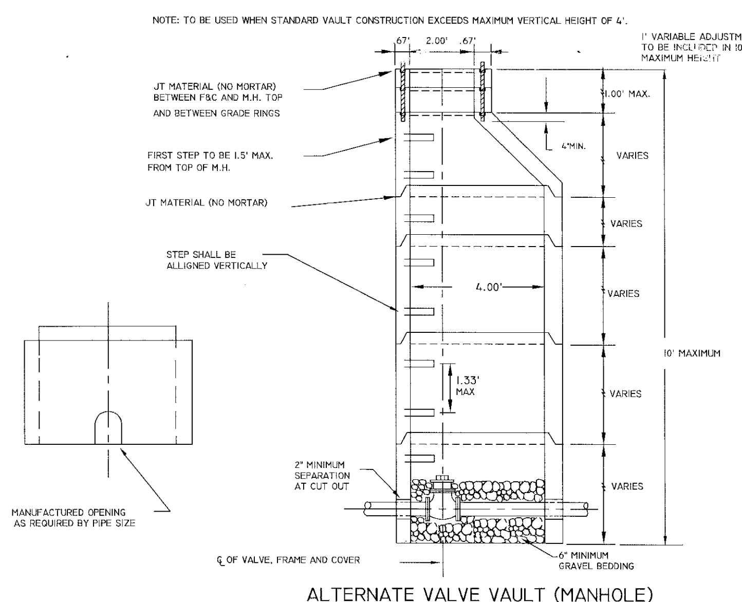
ALTERNATE VALVE VAULT (MANHOLE)
