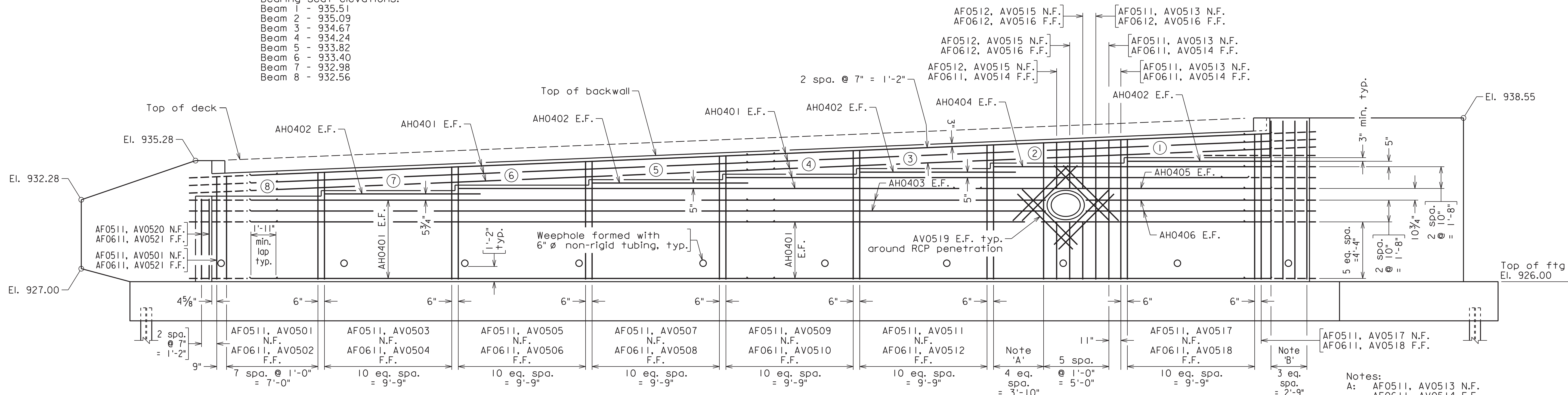
ABUTMENT A ELEVATION Scale: 1/4" = 1'-0"
