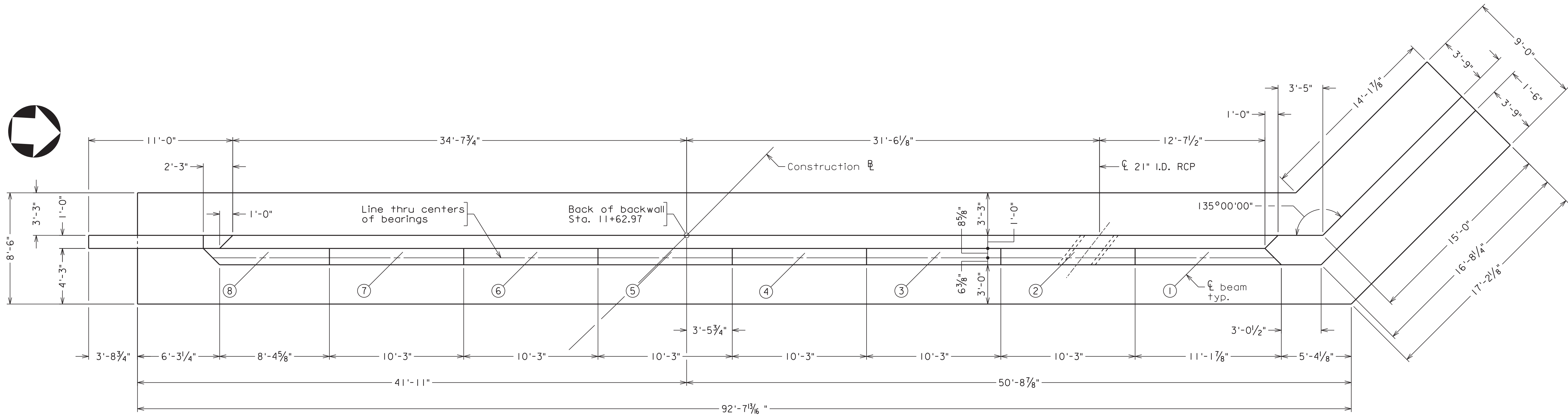
ABUTMENT A PLAN Scale: 1/4" = 1'-0"
