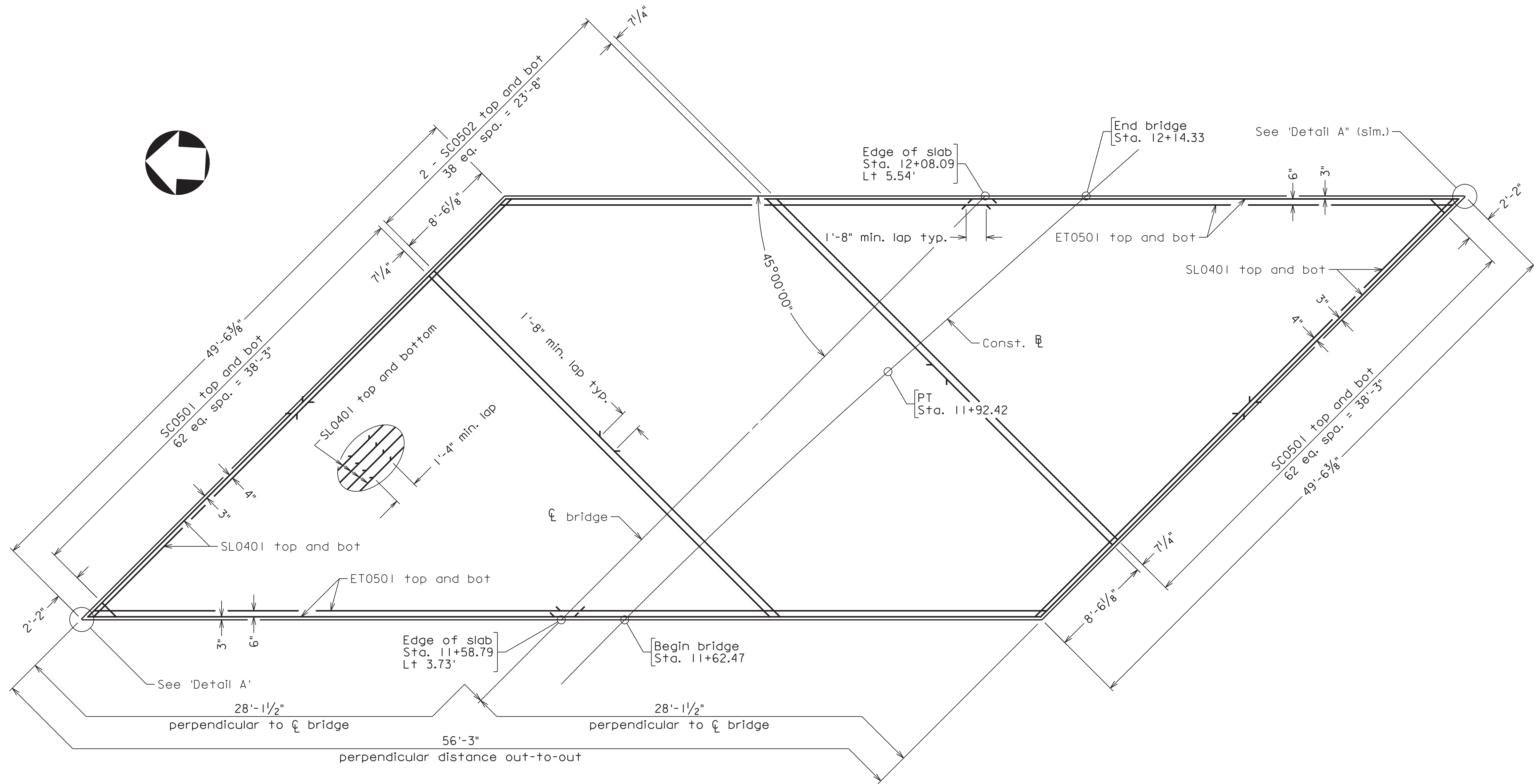
DECK PLAN Scale: 3/16" = 1'-0"
