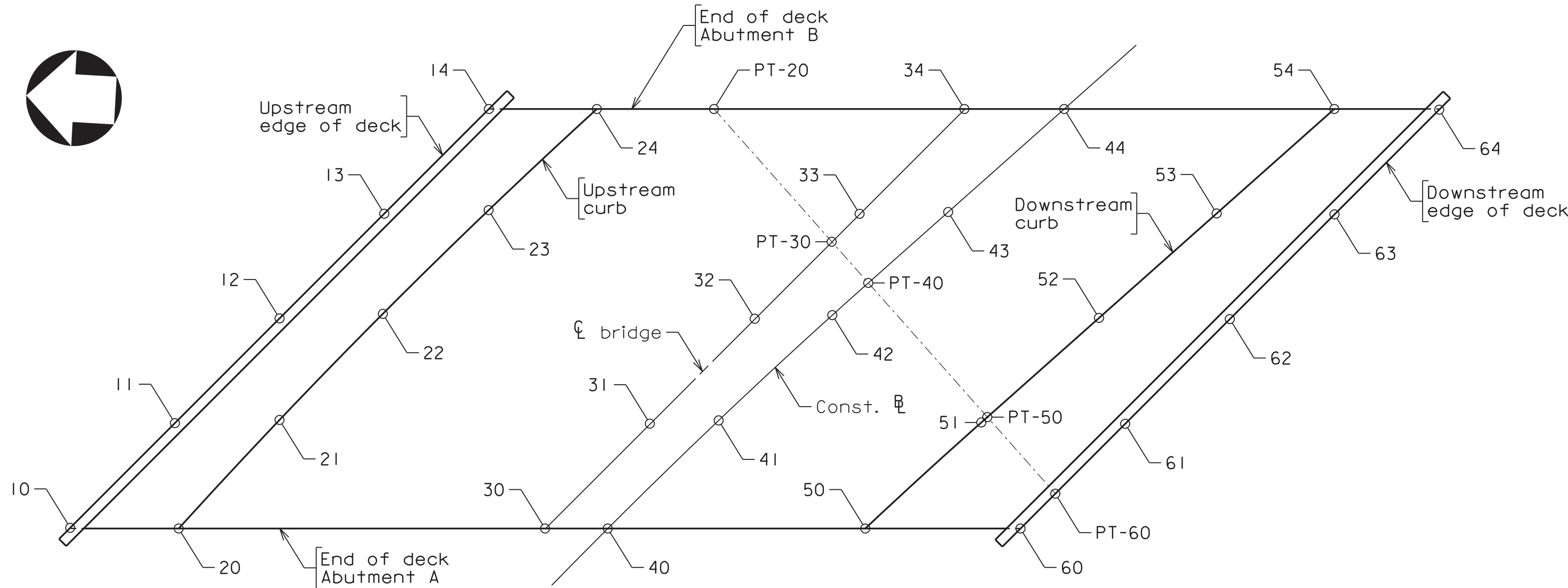
PLAN FOR TOP OF DECK ELEVATIONS Not to scale
