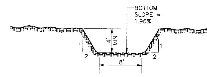
PROPOSED DITCH SECTION C-C N.T.S.
