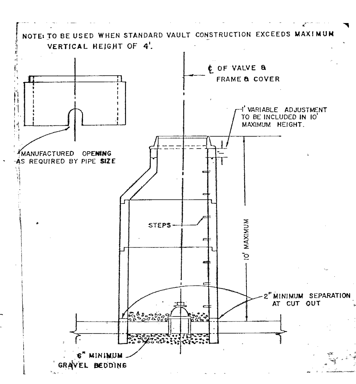
ALTERNATE VALVE VAULT (MANHOLE)
