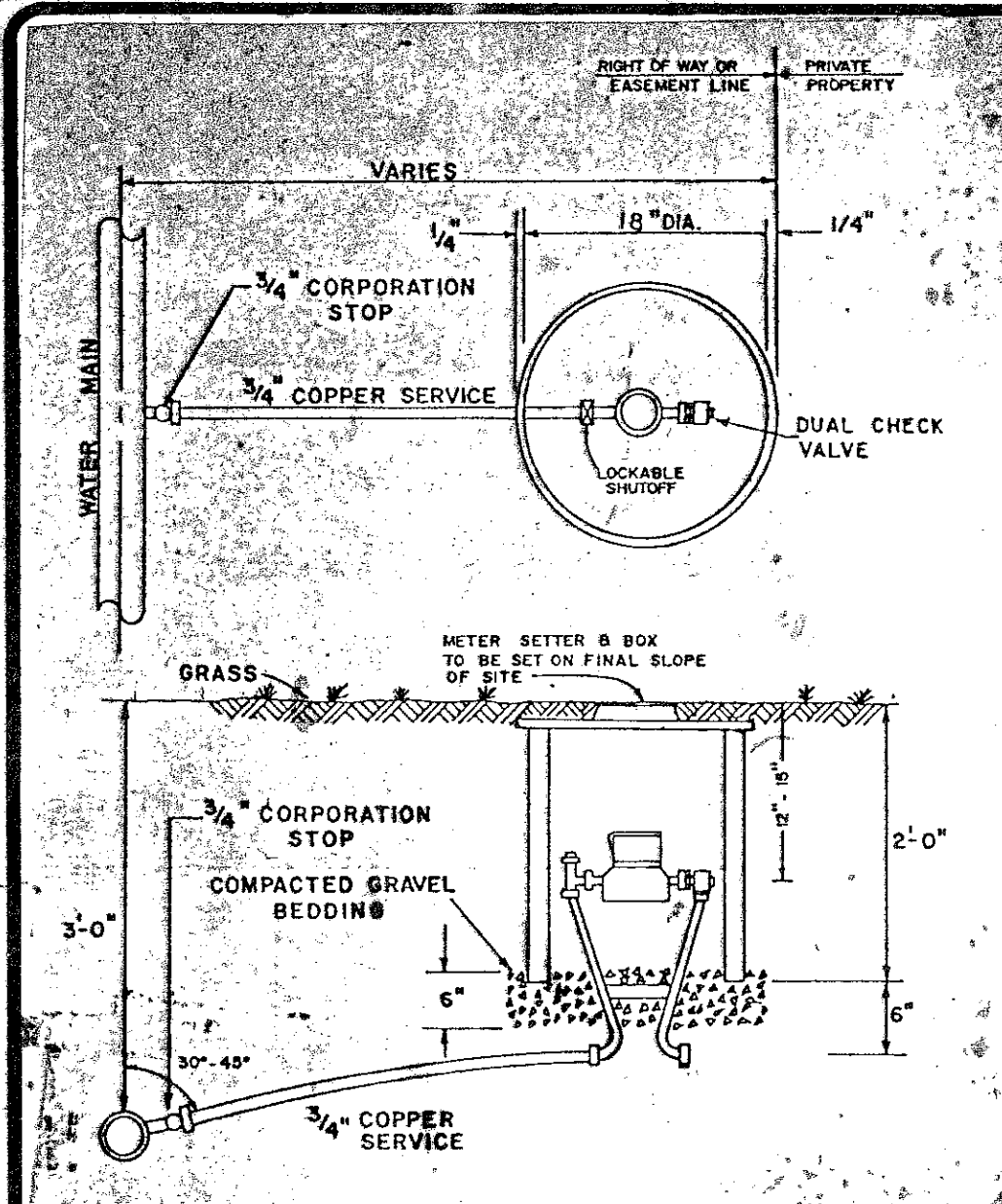
SINGLE RESIDENTIAL WATER SERVICE
