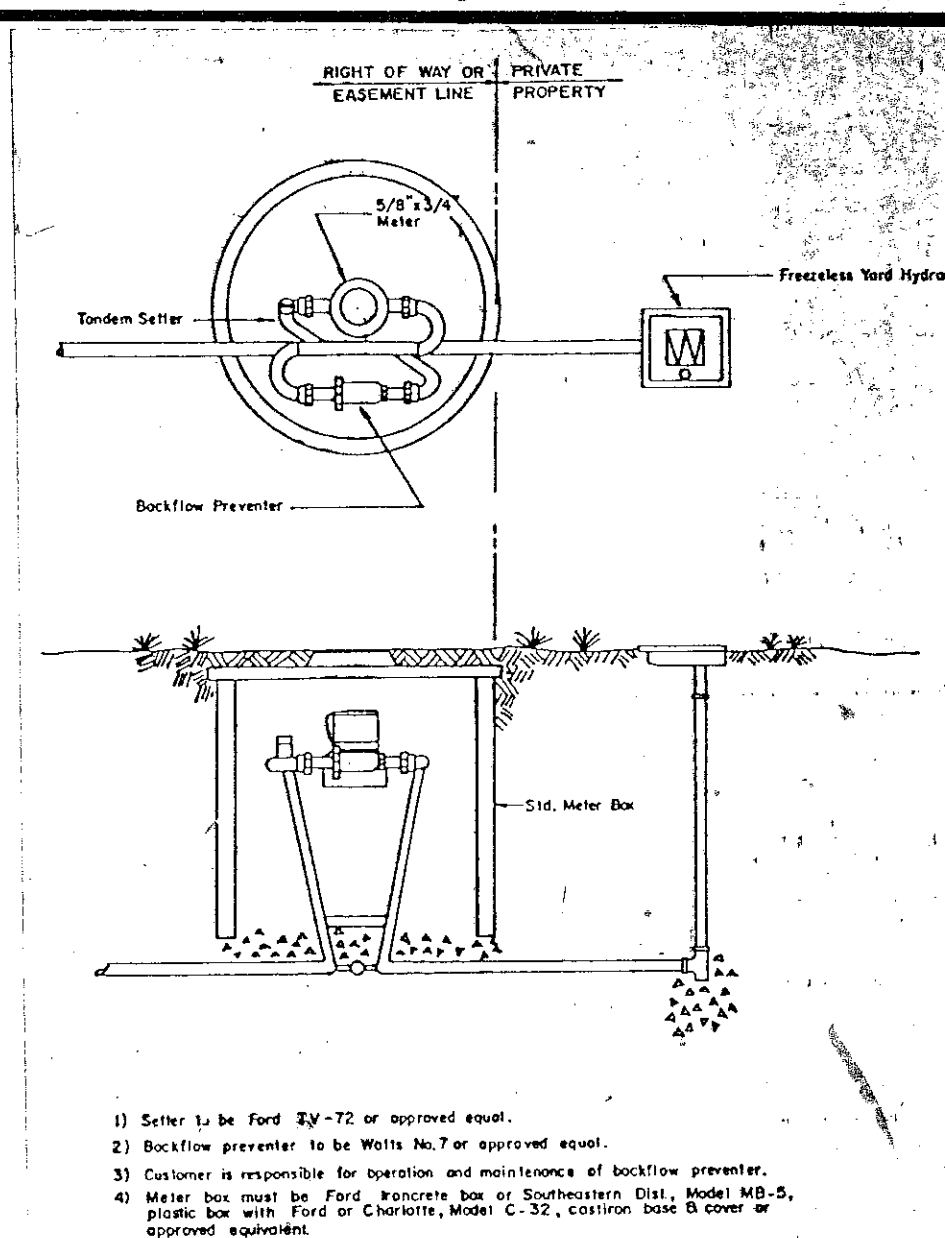
TYPICAL SPRINKLER SERVICE
