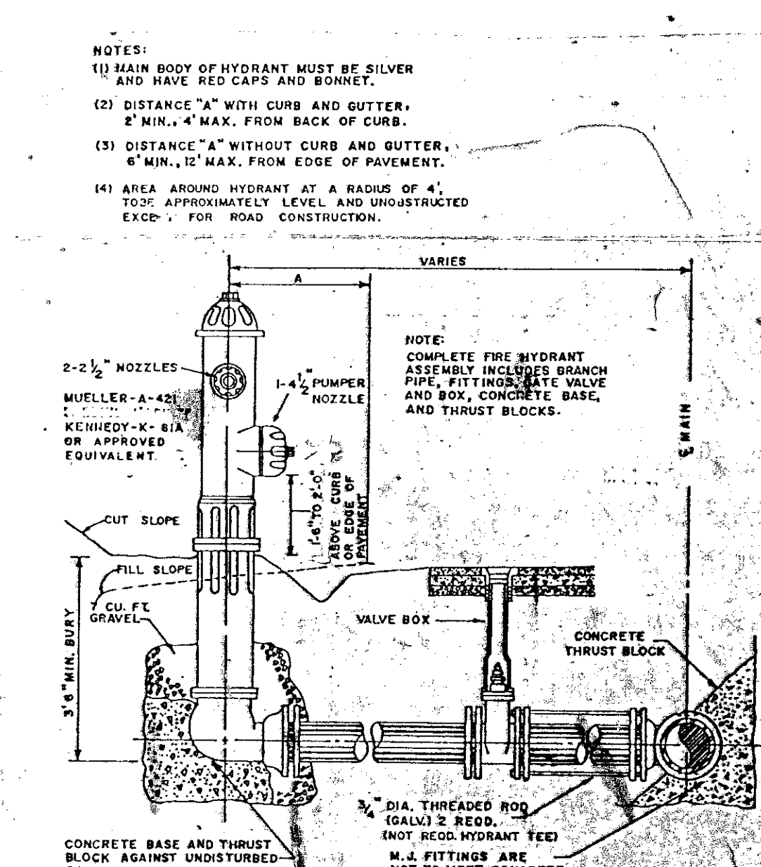
FIRE HYDRANT SETTING
