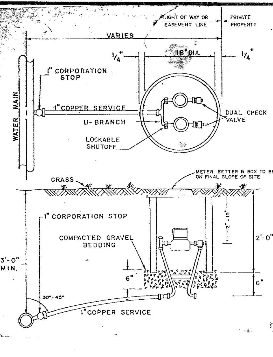
DOUBLE RESIDENTIAL WATER SERVICE
