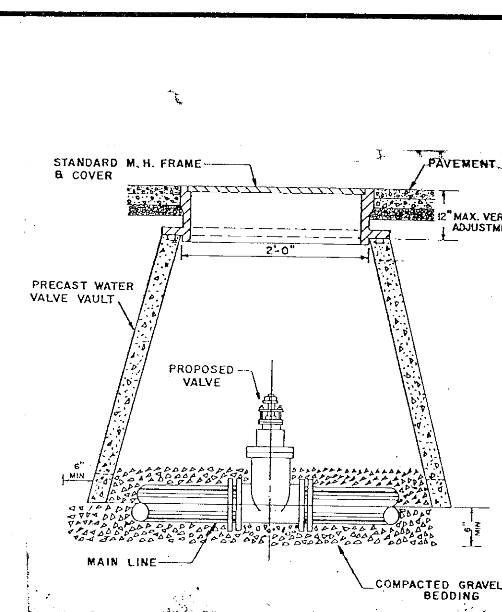
WATER LINE VALVE INSTALLATION
