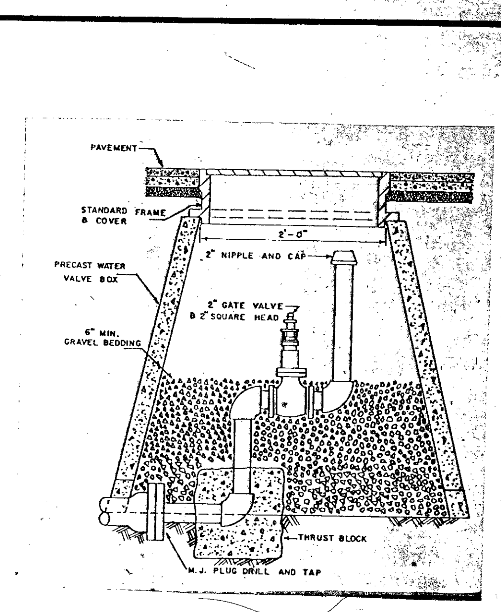
PERMANENT END OF LINE
