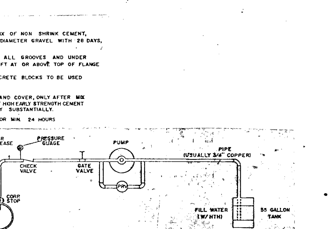
TYPICAL WATER PRESSURE TEST RIG
