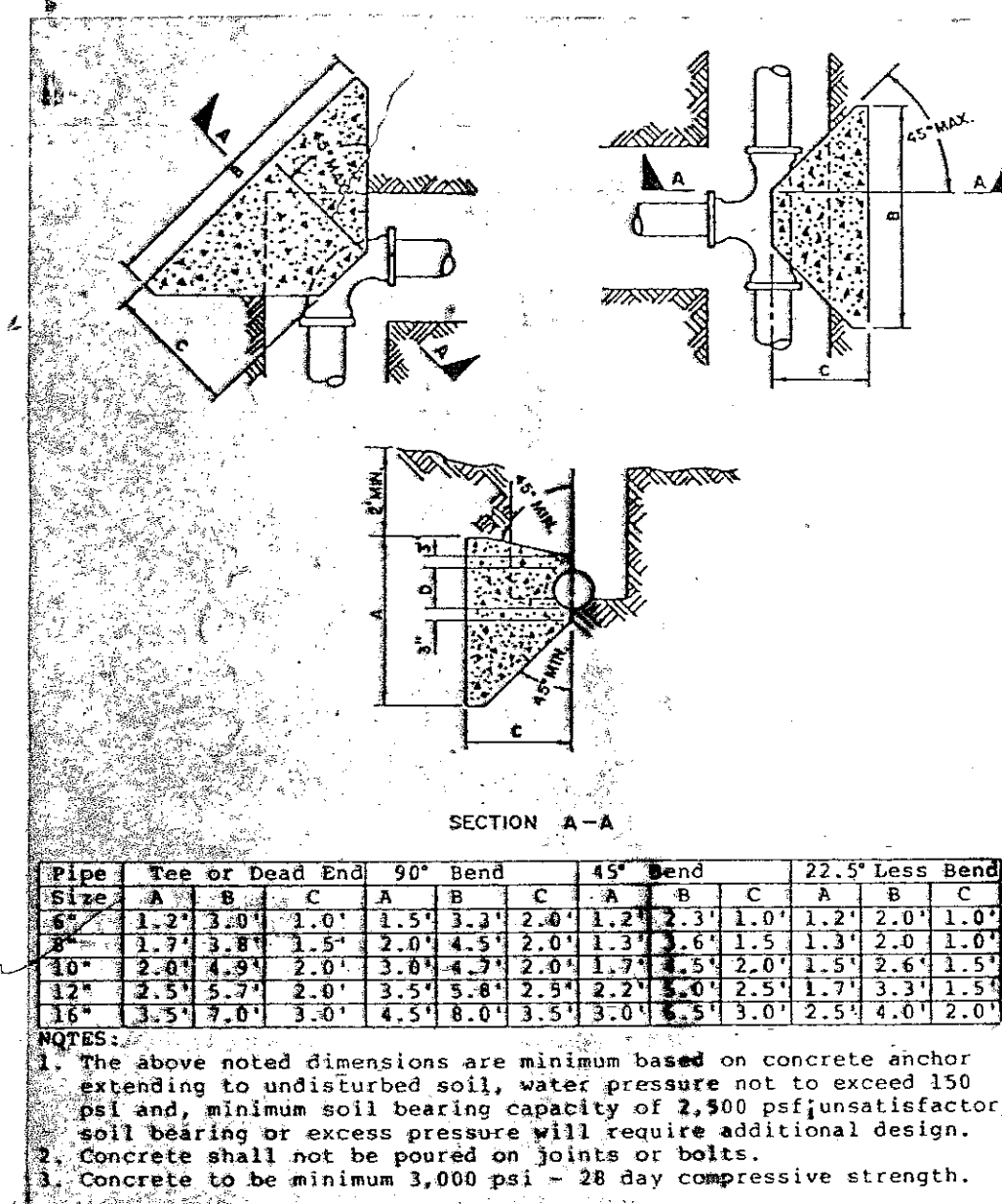
THRUST BLOCK FOR HORIZONTAL & LOWER VERTICAL BENDS
