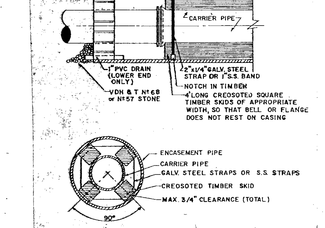
PIPE SUPPORT IN CASING PIPE
