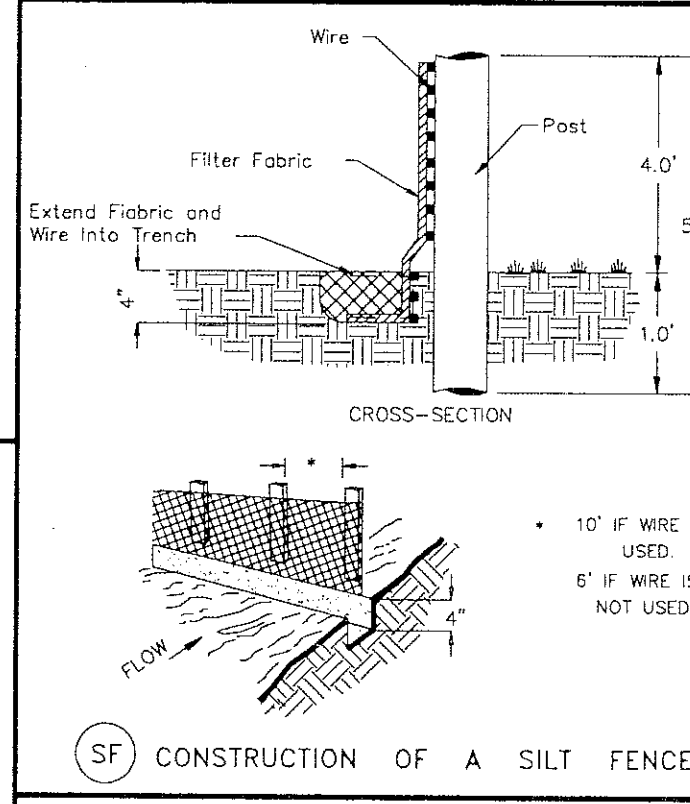
(SF) CONSTRUCTION OF A SILT FENCE
