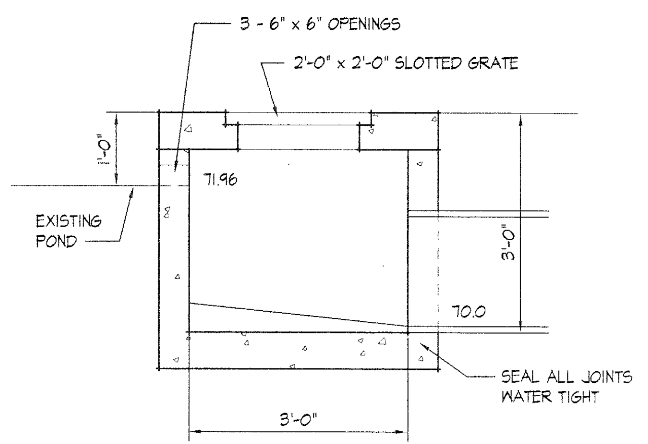
SECTION SCALE 3/4" = 1'-0" C4.1 C4
