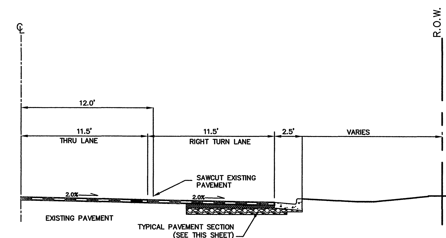
TYPICAL SECTION - COVE ROAD (SECTION #3)
