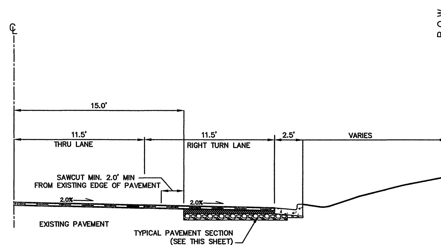
TYPICAL SECTION - COVE ROAD (SECTION #2)
