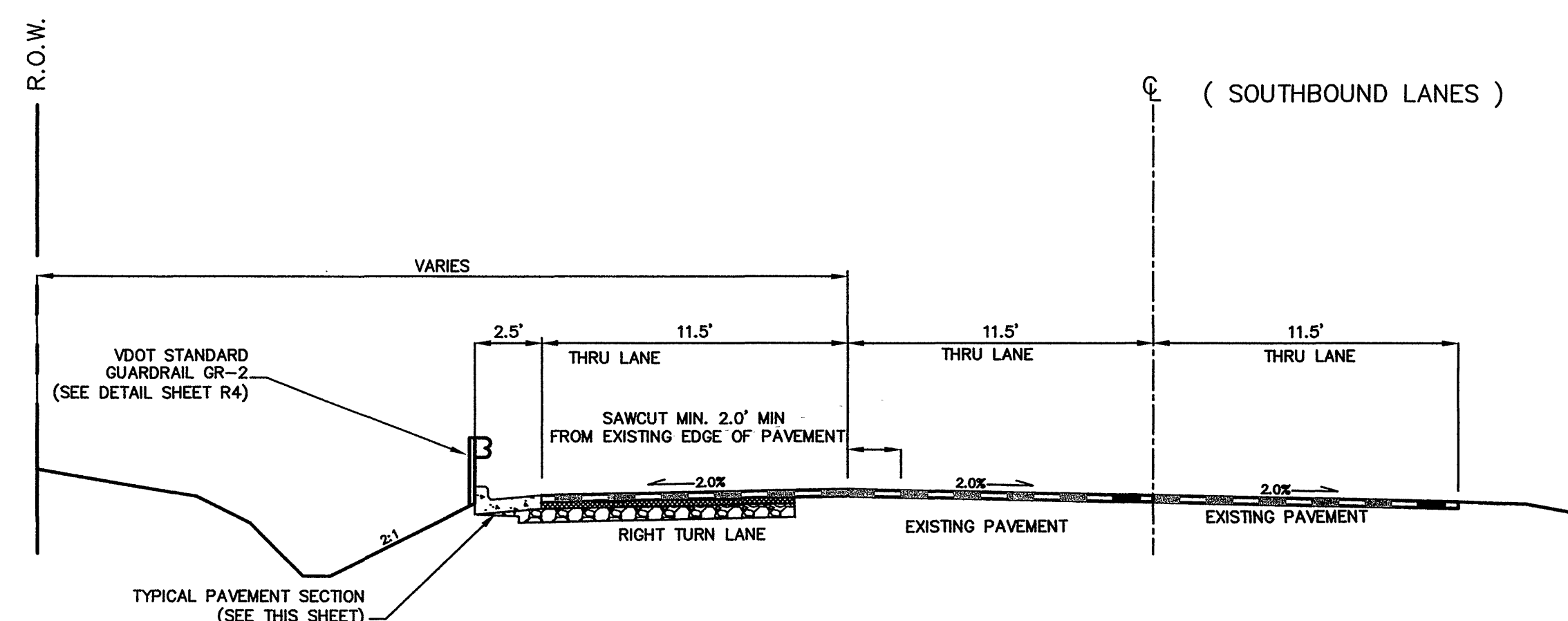
SECTION #3 - PETERS CREEK
