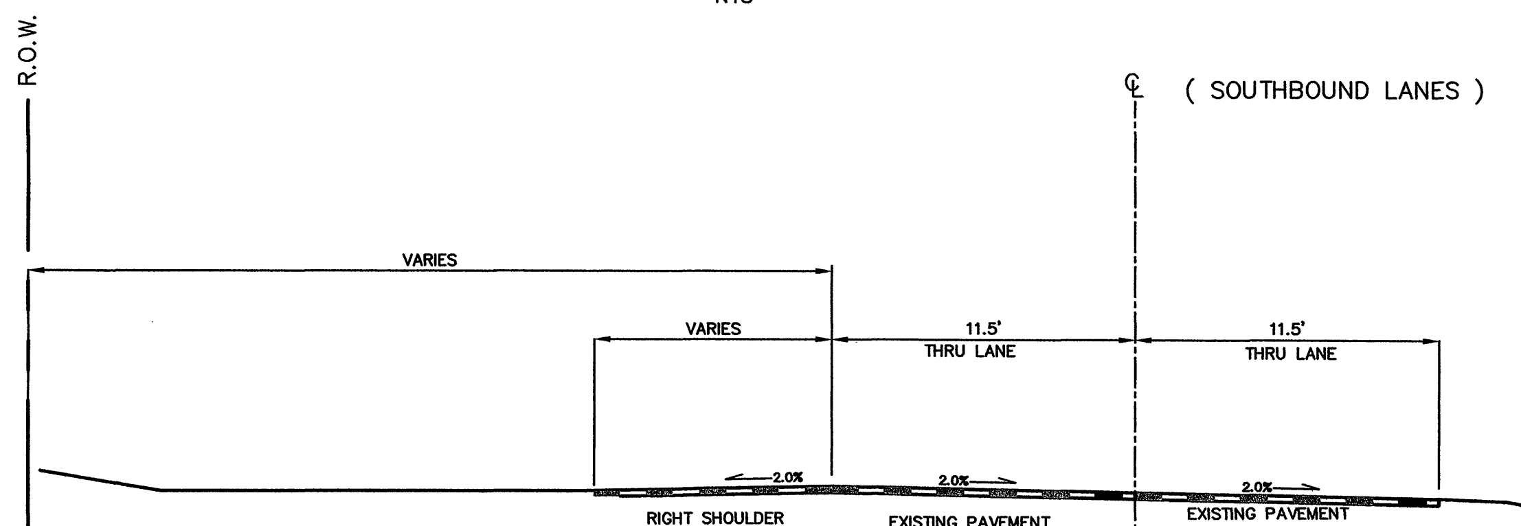
SECTION #2 - PETERS CREEK
