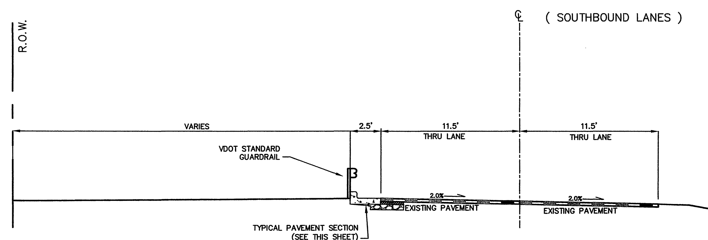
SECTION #1 - PETERS CREEK
