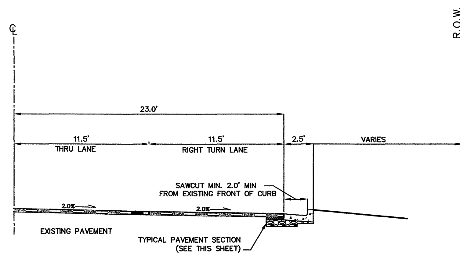
TYPICAL SECTION - COVE ROAD (SECTION #1)
