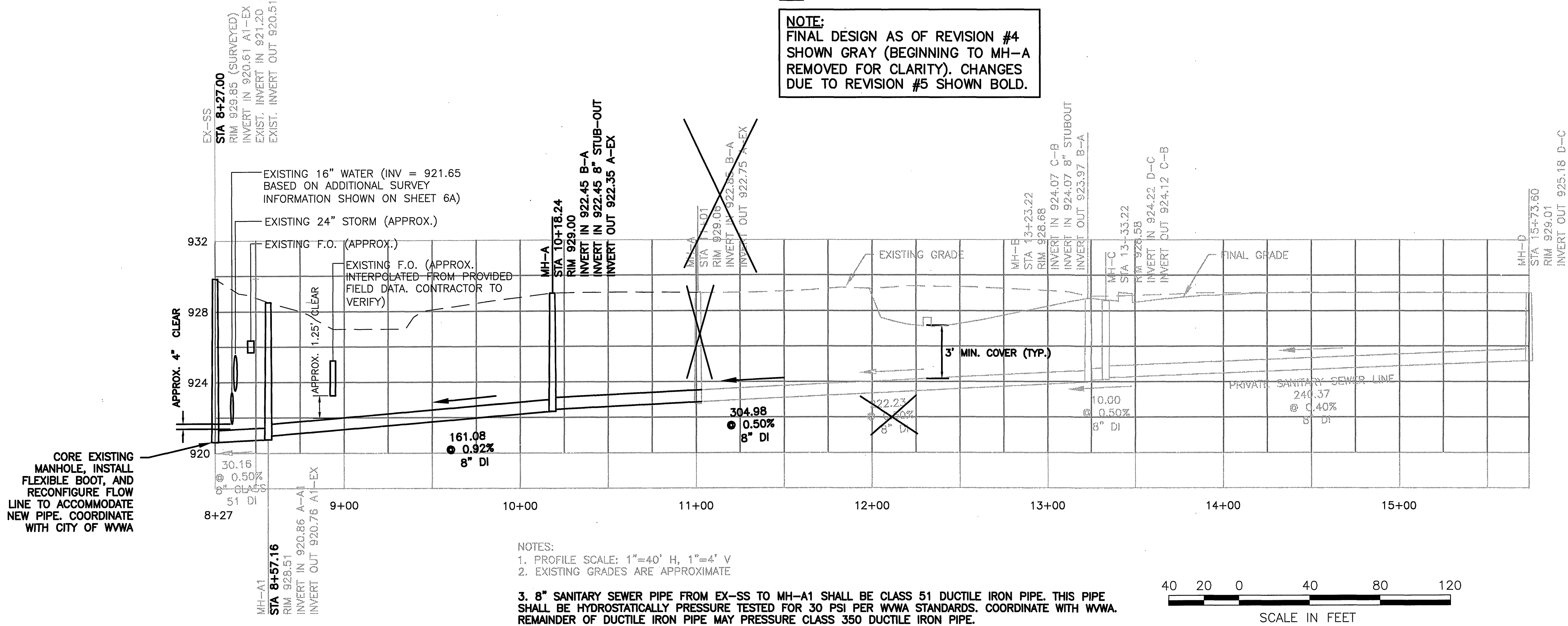
SANITARY SEWER PROFILE STA: 10+00 TO 15+73.60
