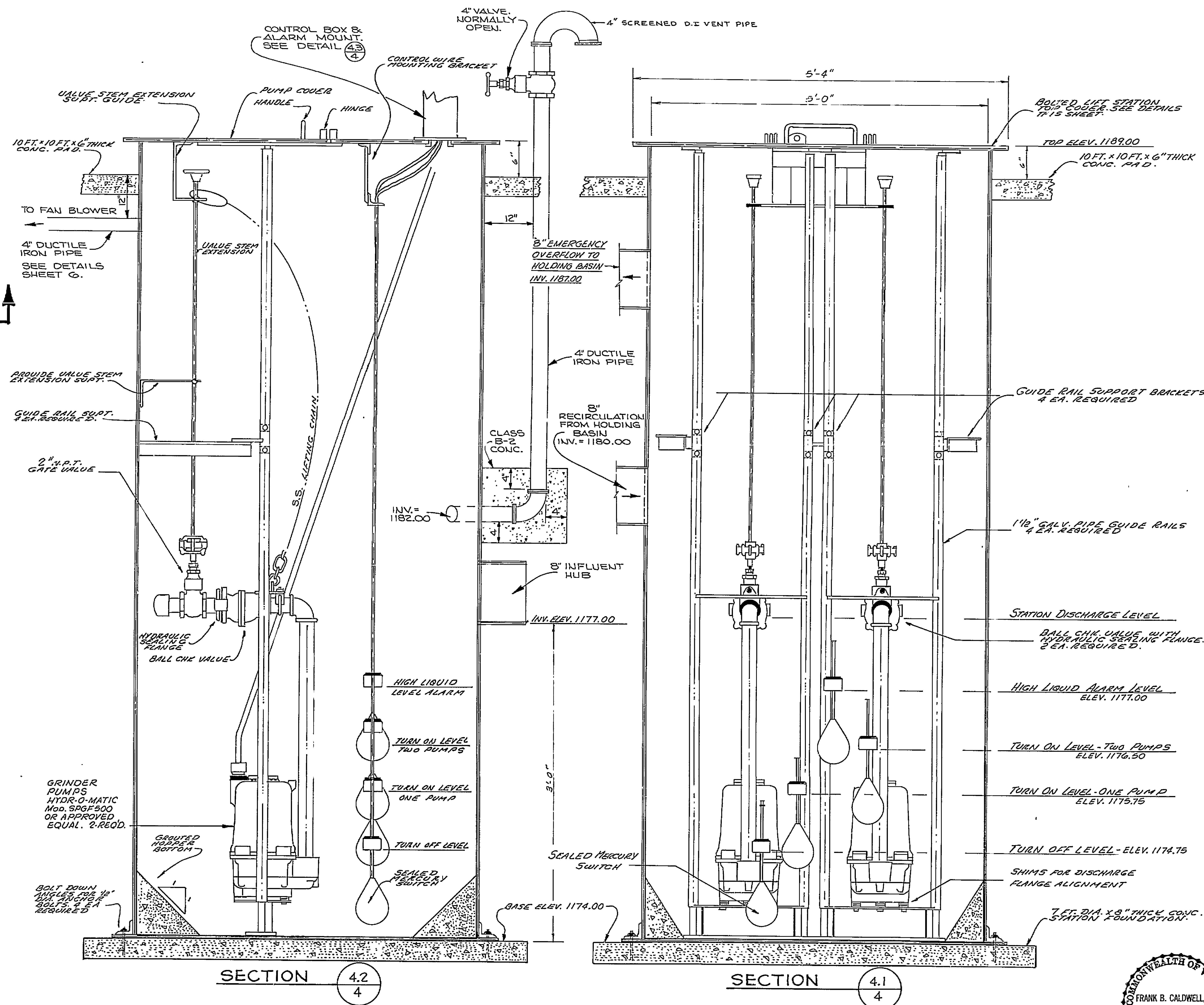
DUPLEX HYDR-O-GRIND SEWAGE PUMP STATION
