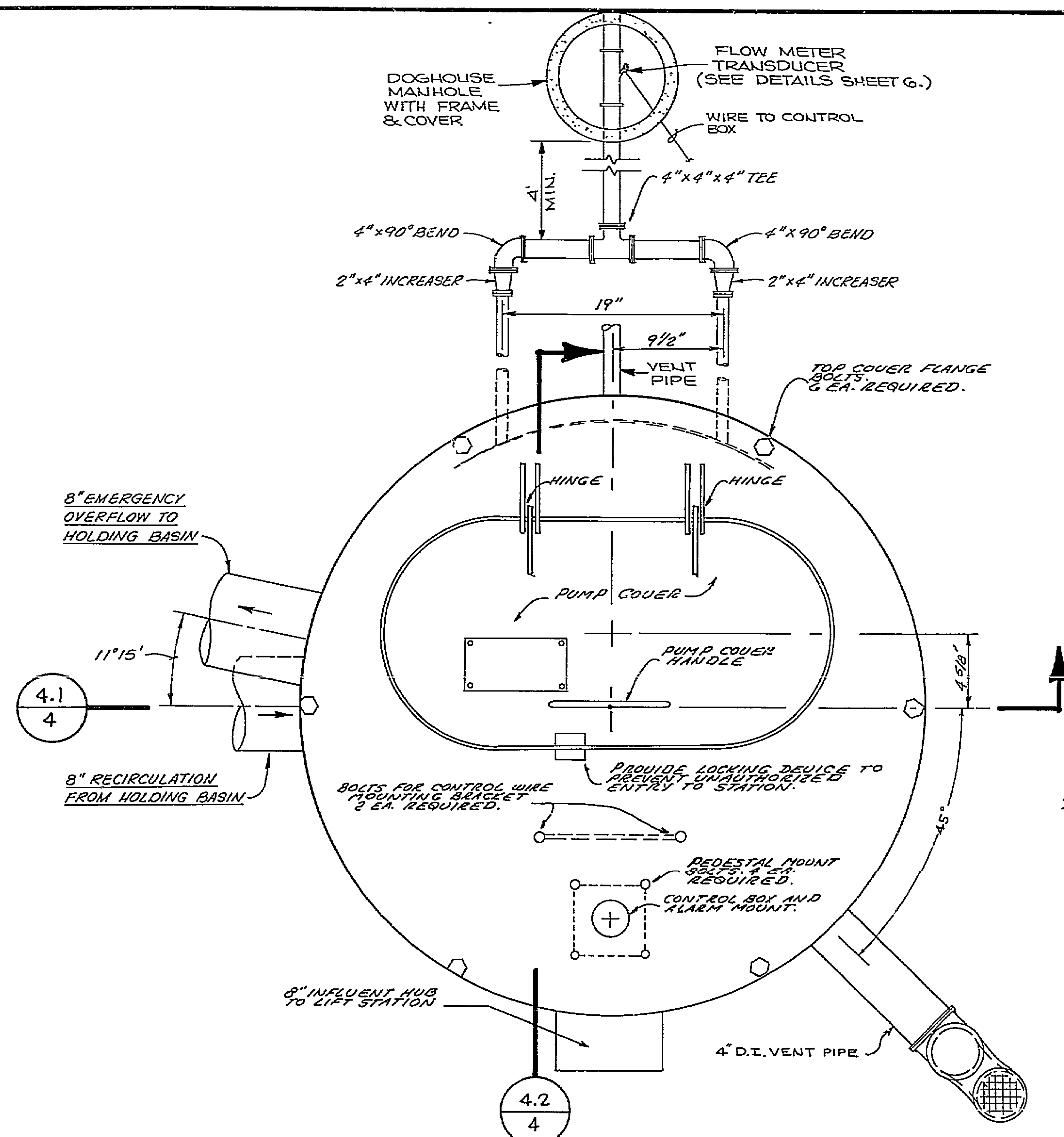
TOP VIEW-LIFT STATION COVER
