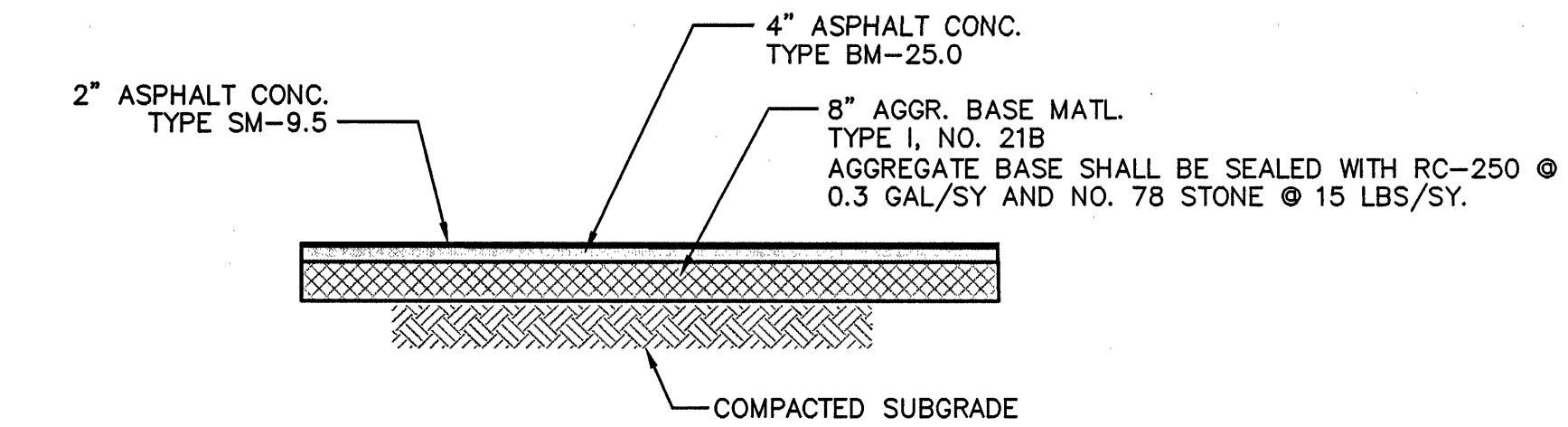
TYPICAL PAVEMENT SECTION - ACCESS ROAD AND TRUCK AREAS NOT TO SCALE
