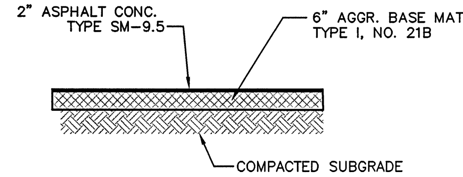
TYPICAL PAVEMENT SECTION - PARKING LOT (ONLY) NOT TO SCALE
