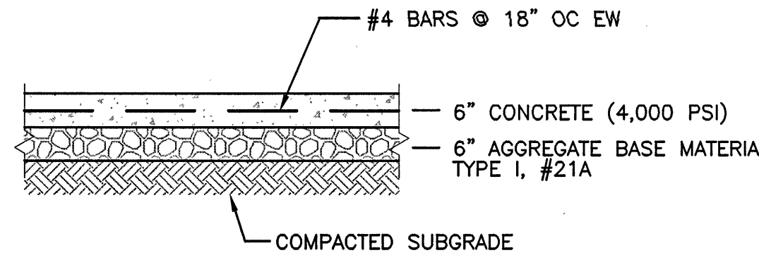
NOTE: SPECIFICATION SECTION 02514 FOR JOINTS. TYPICAL CONCRETE PAVING SECTION AND LANDING GEAR PADS NO SCALE
