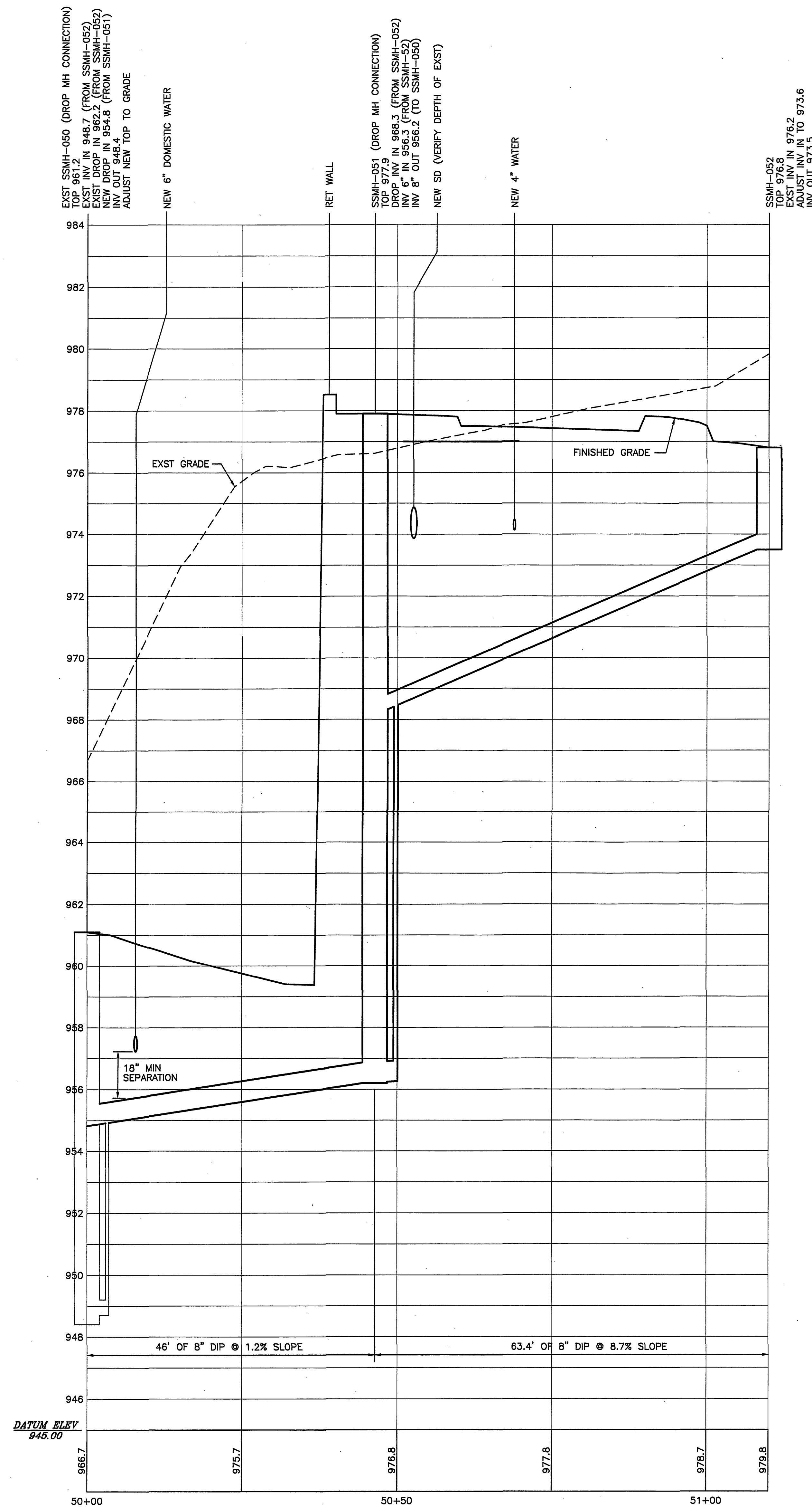
SANITARY SEWER 050 TO 052 PROFILE SCALE HORIZ. 1"=10' VERT. 1"=2'
