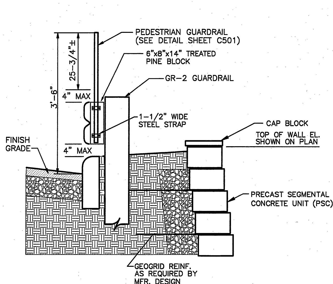
PEDESTRIAN GUARDRAIL/GR-2 GUARDRAIL NO SCALE
