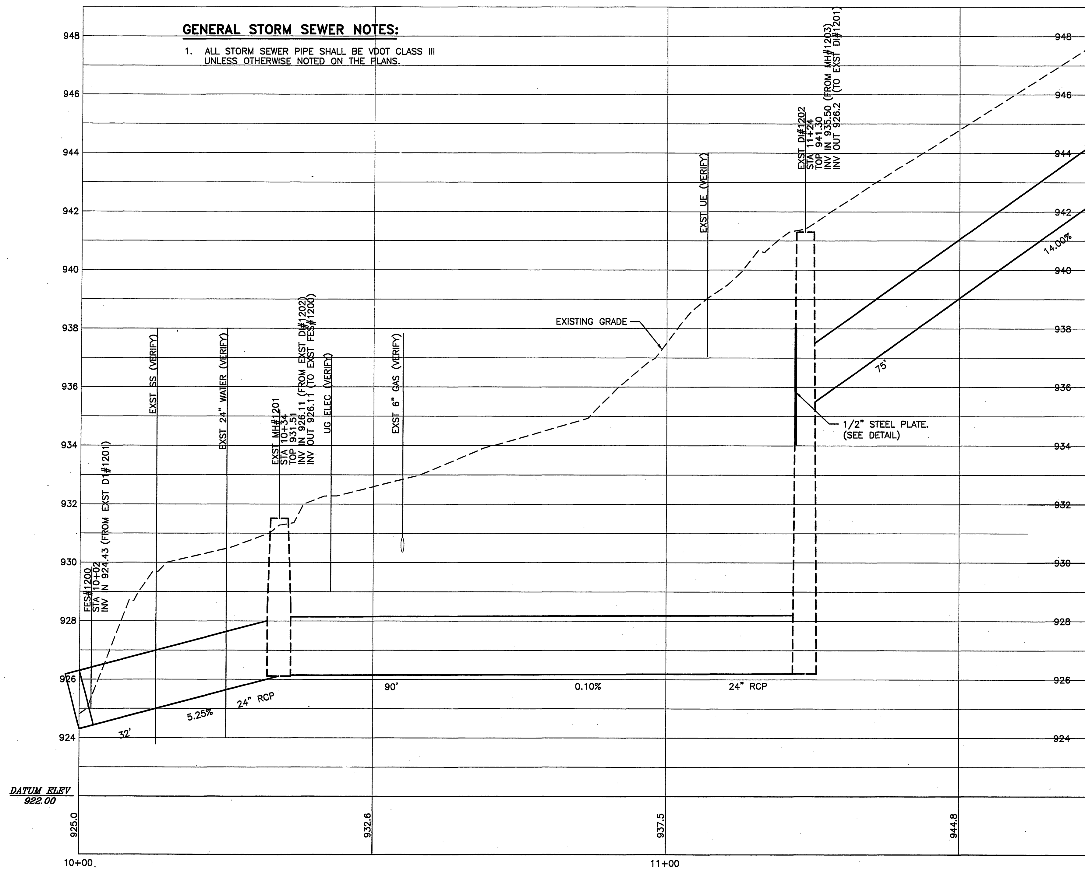
STORM DRAIN FES#1200 TO DI#1212 PROFILE
