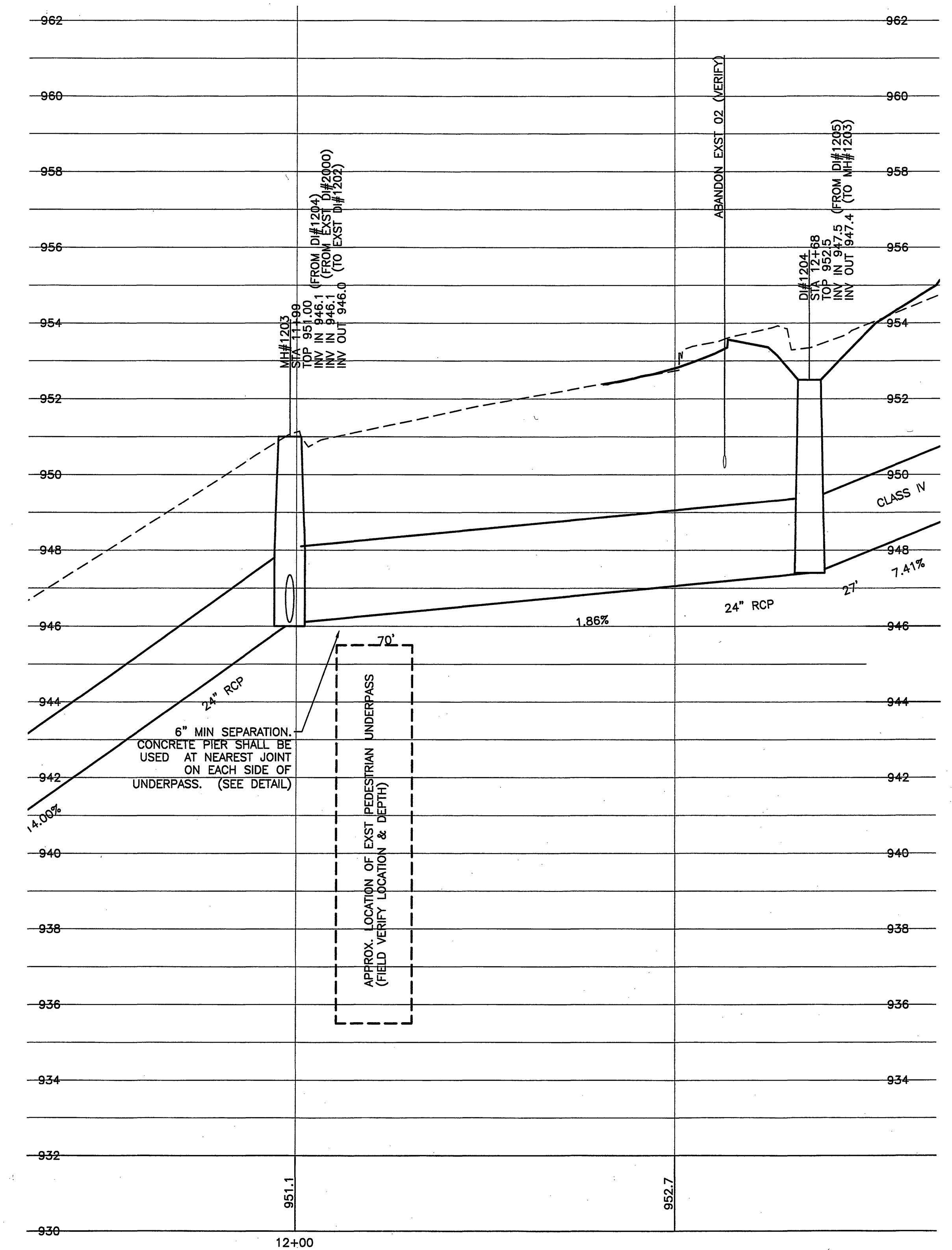
STORM DRAIN FES#1200 TO DI#1212 PROFILE
