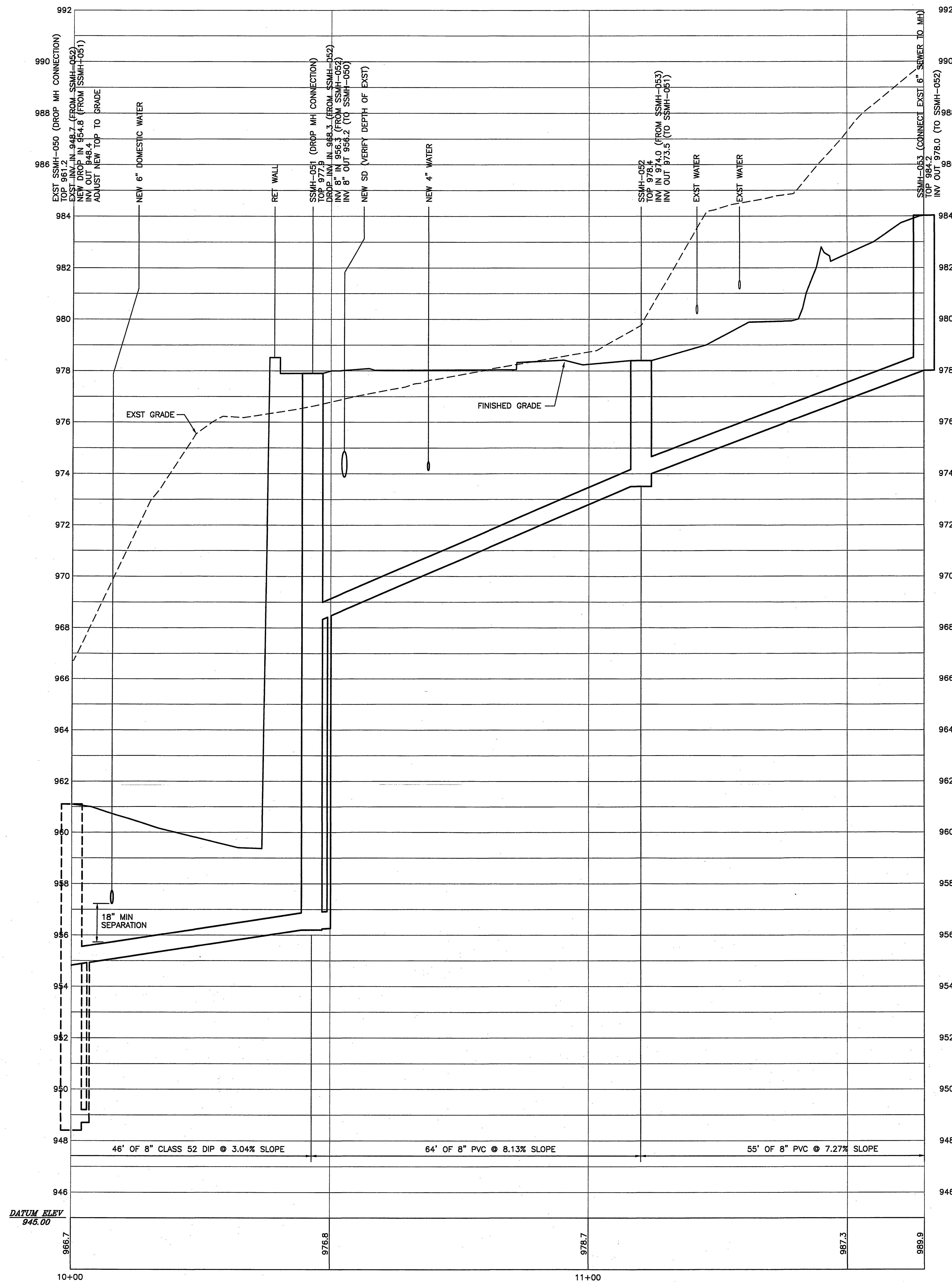
SANITARY SEWER 050 TO 053 PROFILE SCALE: HORIZ. 1"=10' VERT. 1"=2'
