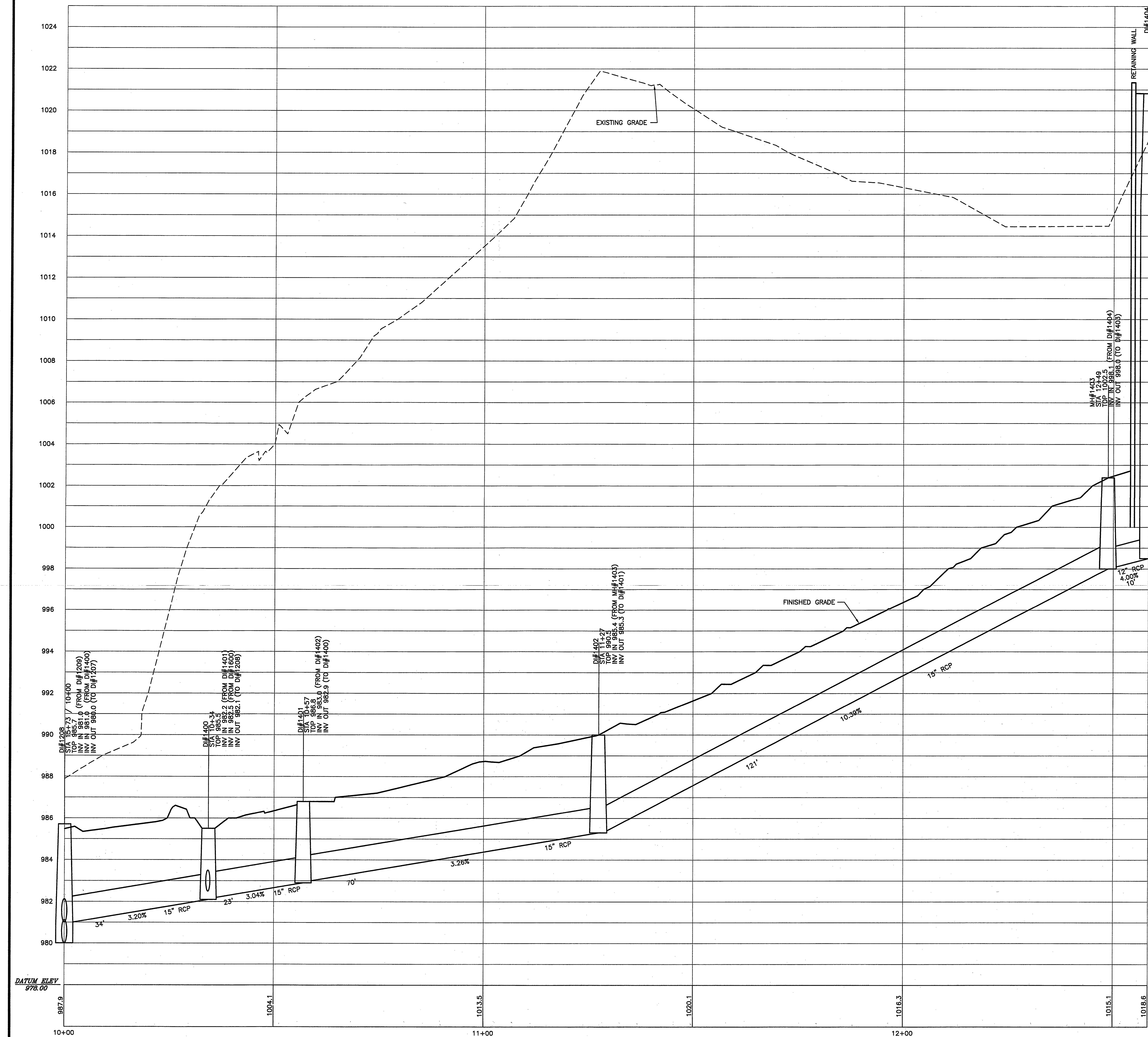
STORM DRAIN DI#1208 TO DI#1404 PROFILE
