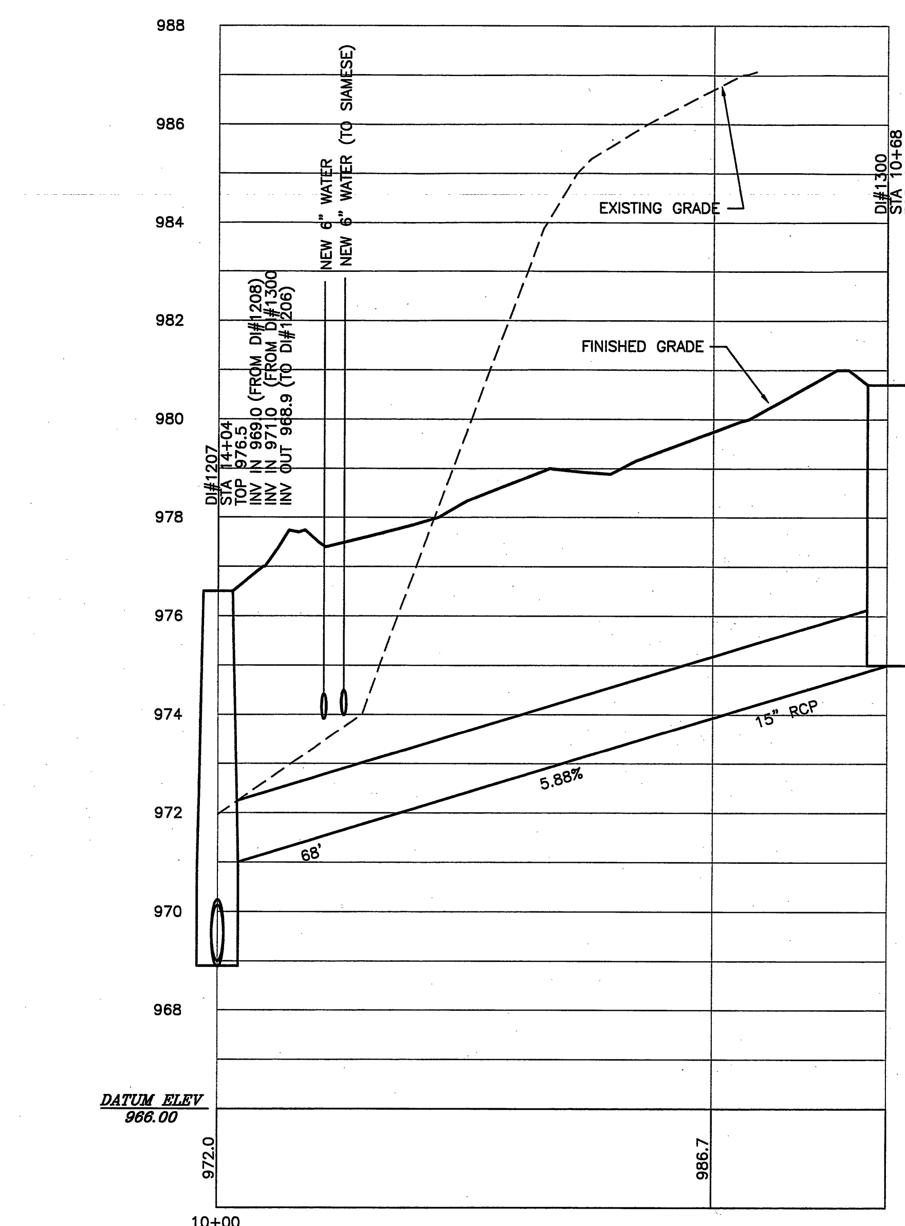
STORM DRAIN DI#1207 TO DI#1300 PROFILE
