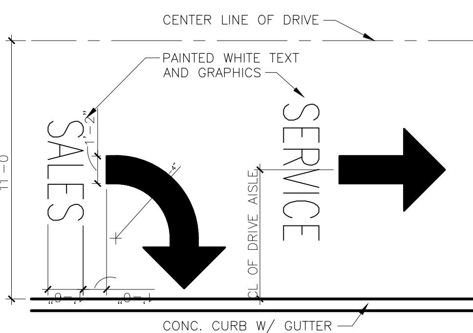
6 DIRECTIONAL SIGNAGE C22.0 SCALE: 1/4" = 1'-0"
