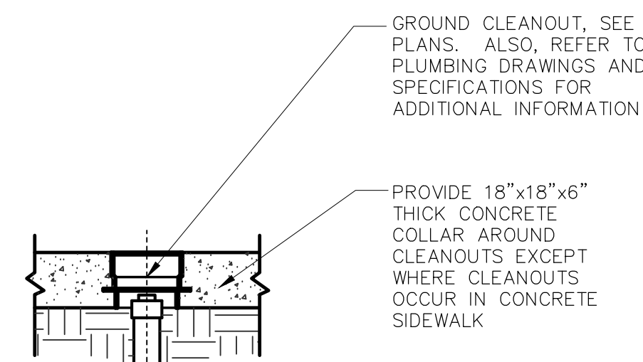
5 TYP. CLEANOUT DTL C22.0 SCALE: 3/4" = 1'-0"
