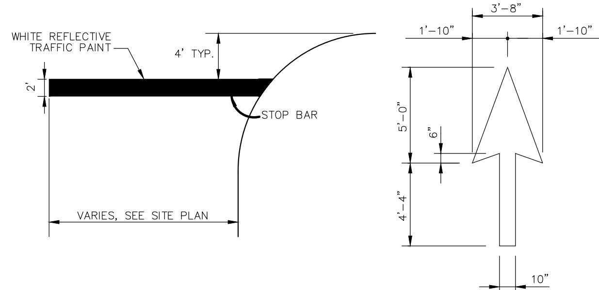
TYP. OFF SITE PAVEMENT AREA MARKINGS N.T.S.
