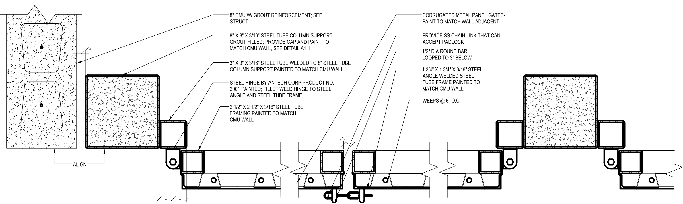
1 HINGE AND LATCH DETAILS C22.0 2" = 1'-0"
