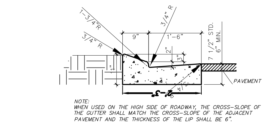
4 TYP. MOUNTABLE CURB C22.0 SCALE: 3/4" = 1'-0"
