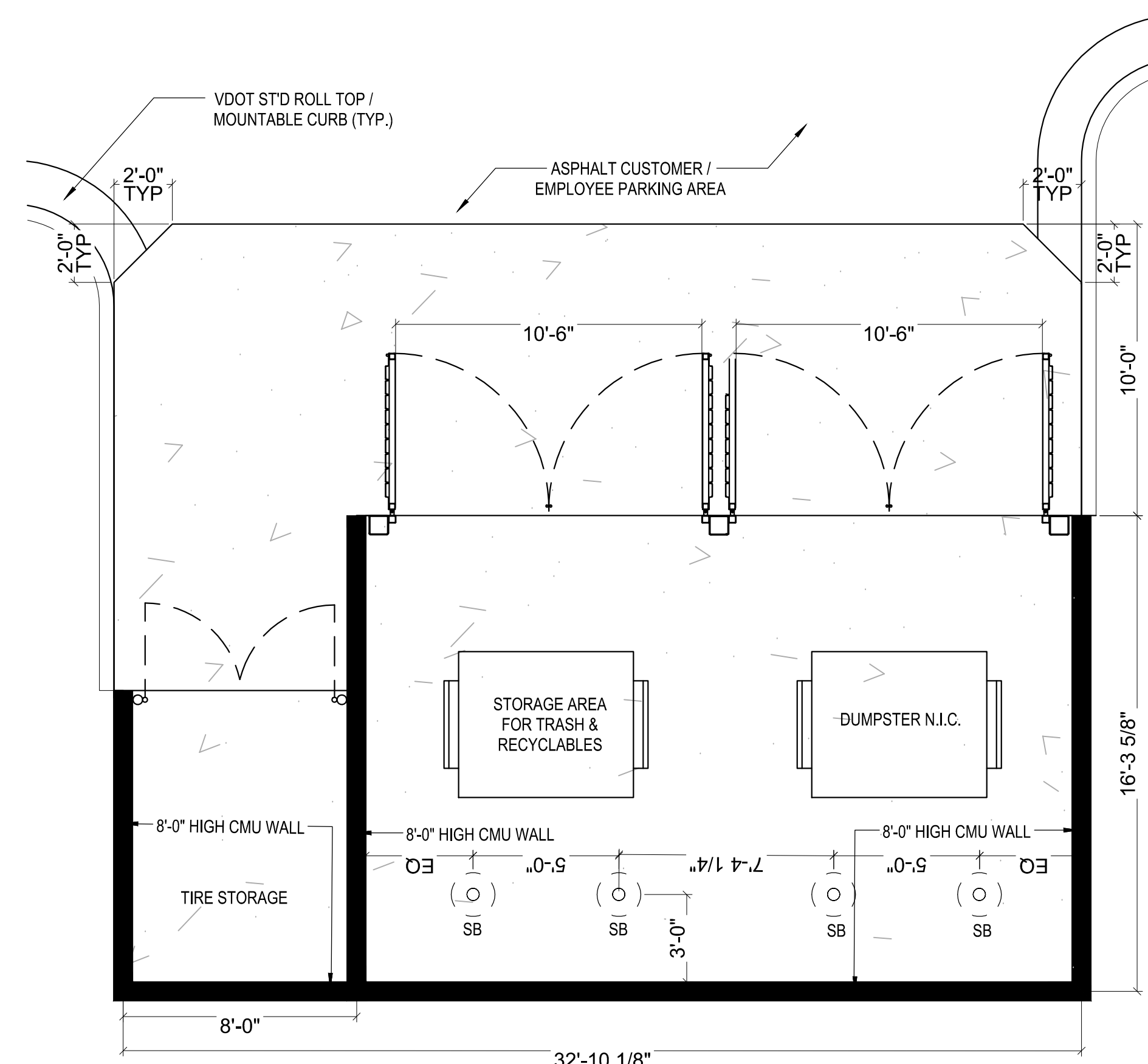
15 DUMPSTER AND TIRE ENCLOSURE PLAN C22.0 SCALE: 1/4" = 1'-0"
