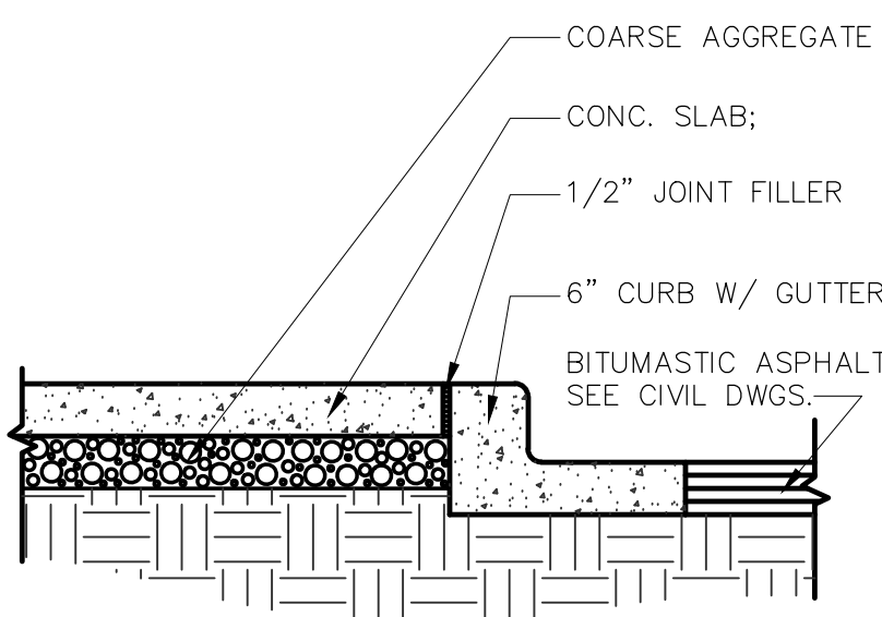
3 TYP. SIDEWALK @ CURB C22.0 SCALE: 3/4" = 1'-0"
