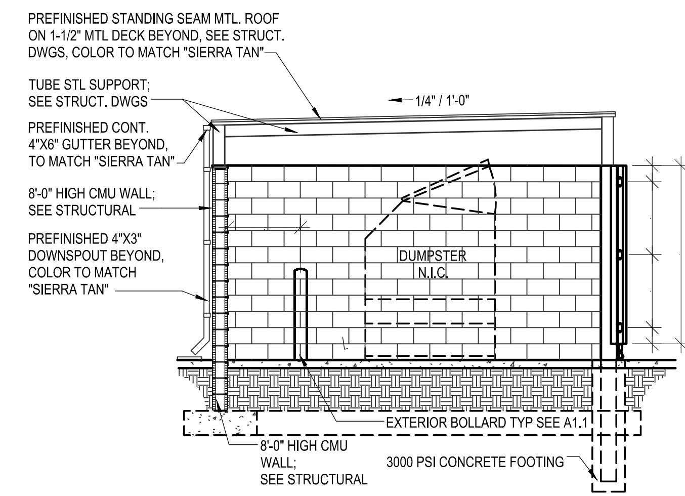
10 SECTION @ DUMPSTER ENCLOSURE C22.0 2" = 1'-0"
