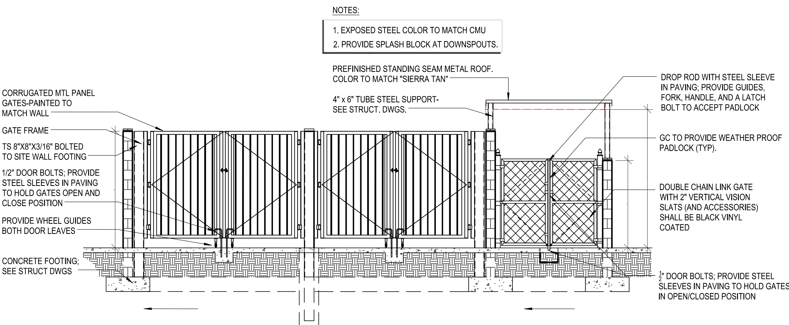
9 ELEVATION - DUMPSTER & TIRE ENCLOSURE C22.0 1/4" = 1'-0"
