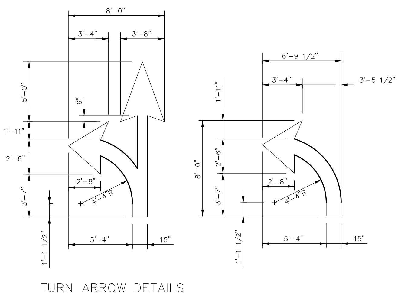
TYP. OFF SITE PAVEMENT AREA MARKINGS N.T.S.
