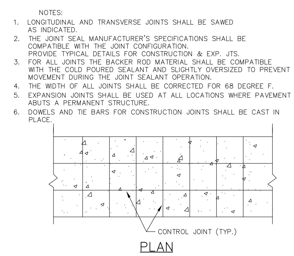
17 DETAIL - CONCRETE PAVEMENT C22.0 SCALE: 1/4" = 1'-0"
