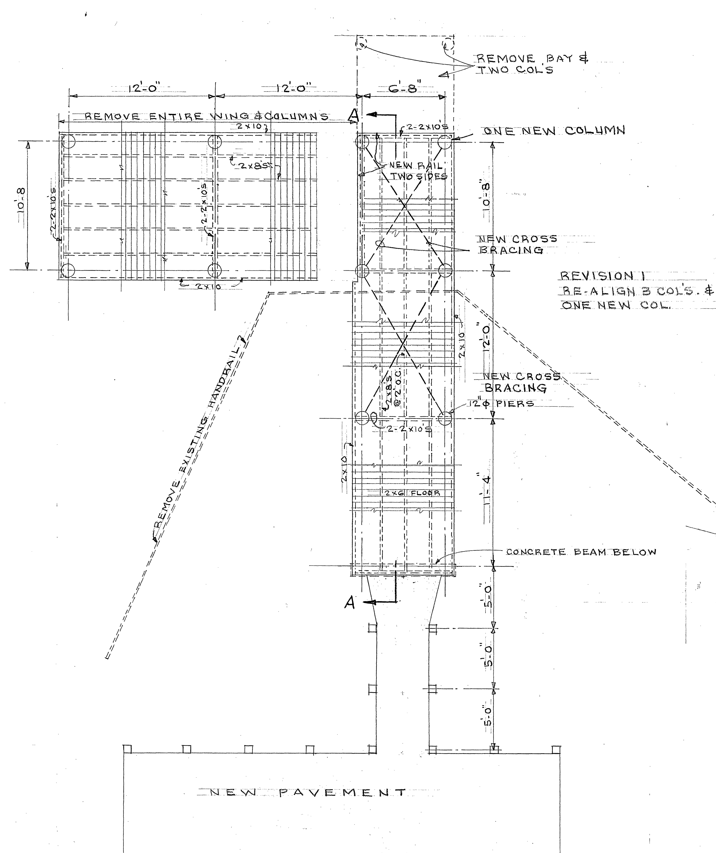
PLAN OF PIER AND RELATED WORK SCALE: 1/4" = 1'-0"
