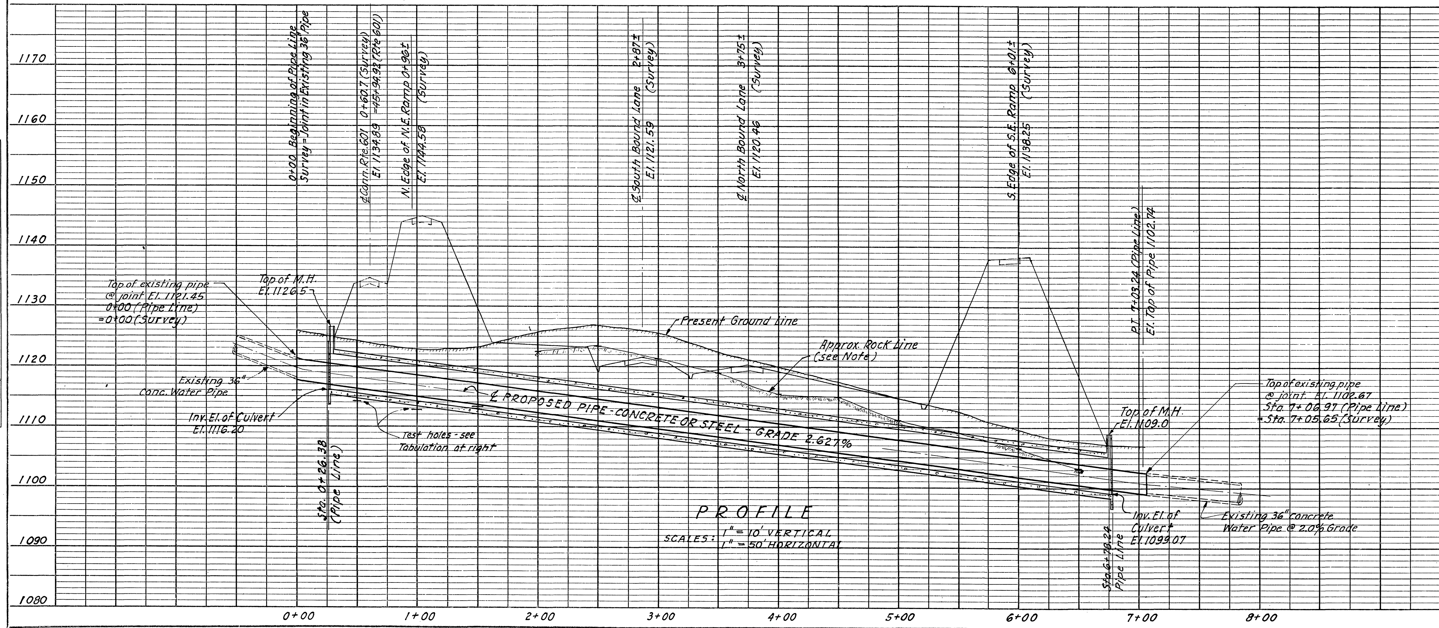
TEST HOLES ON SURVEY LINE
