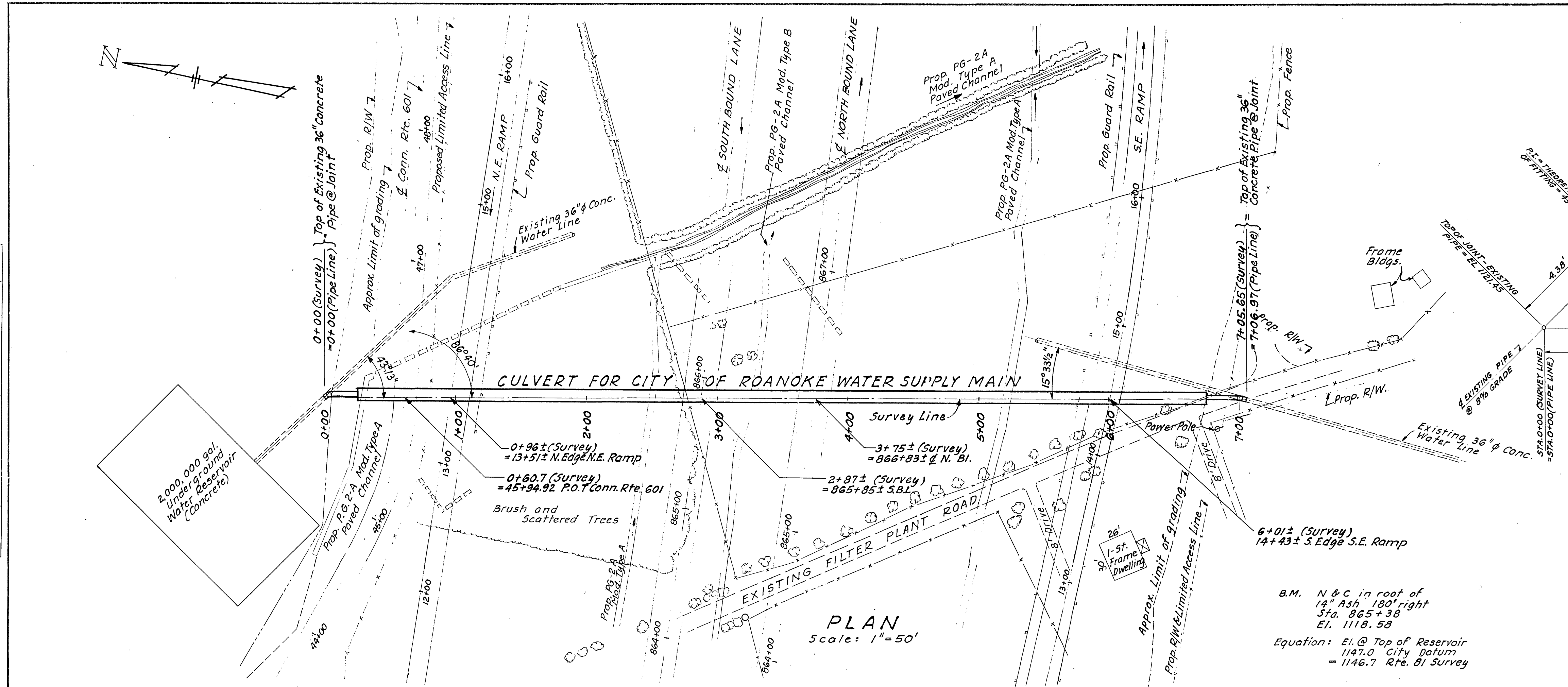
SCHEMATIC DIAGRAM-PIPE LINE & CULVERT
