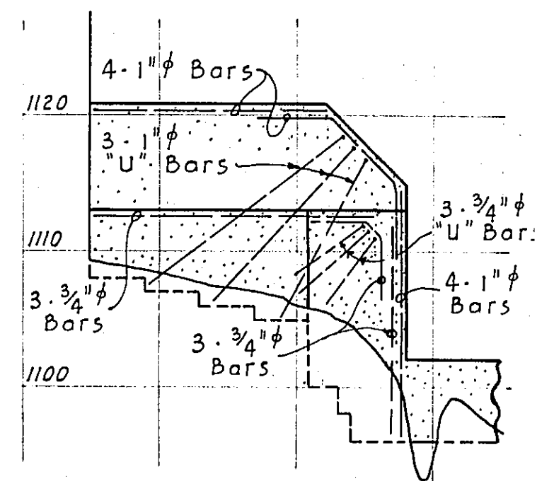
REINFORCING FOR CONCRETE ENCASEMENT
