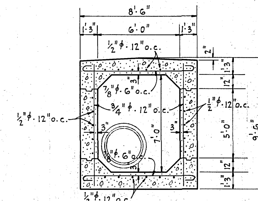
TUNNEL SECTION
