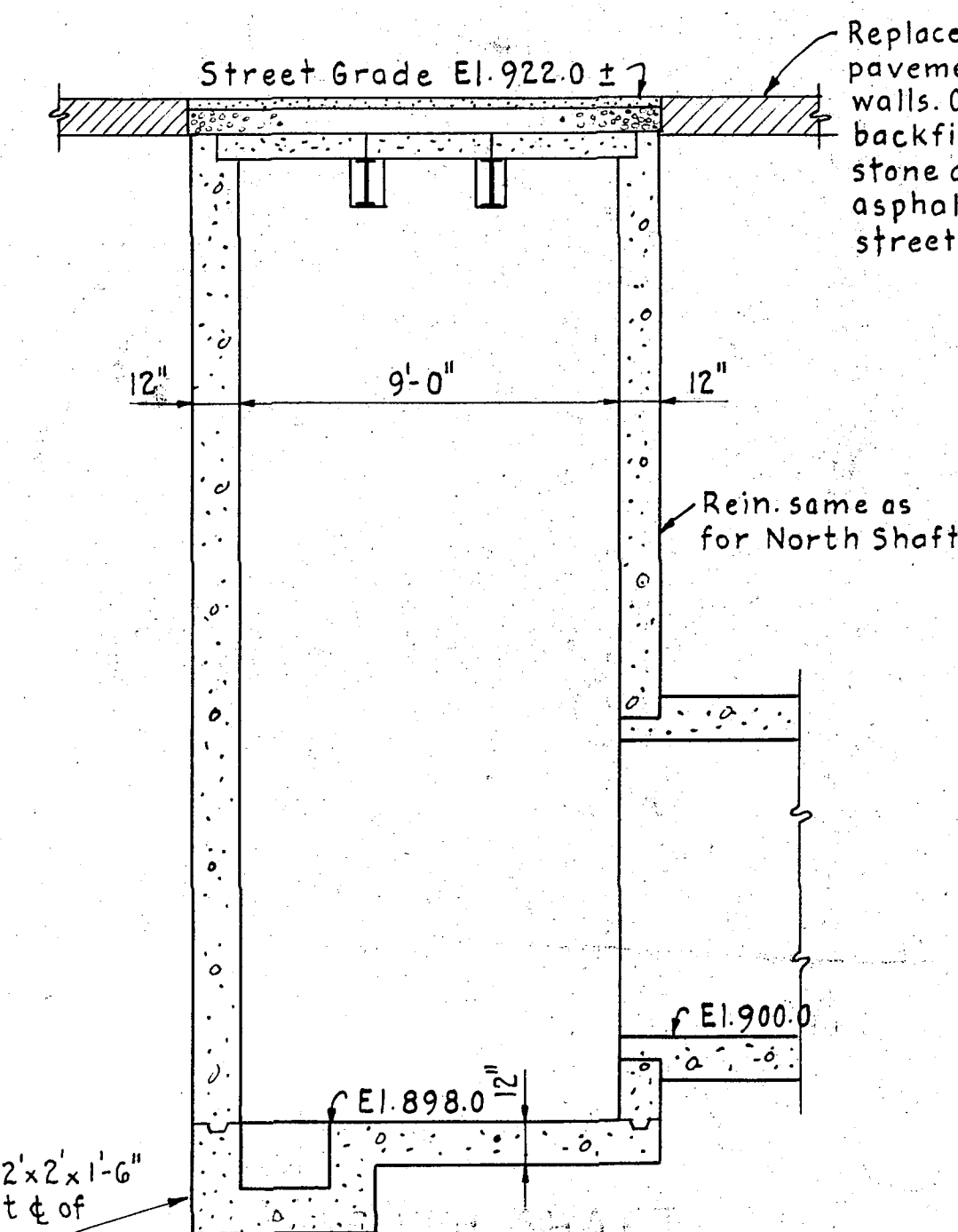
SOUTH SHAFT
