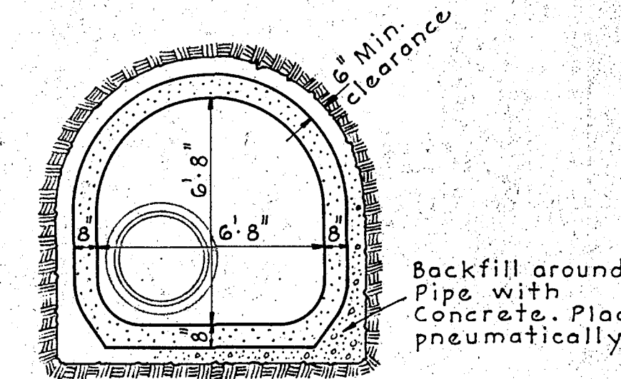
ALTERNATE TUNNEL SECTION
