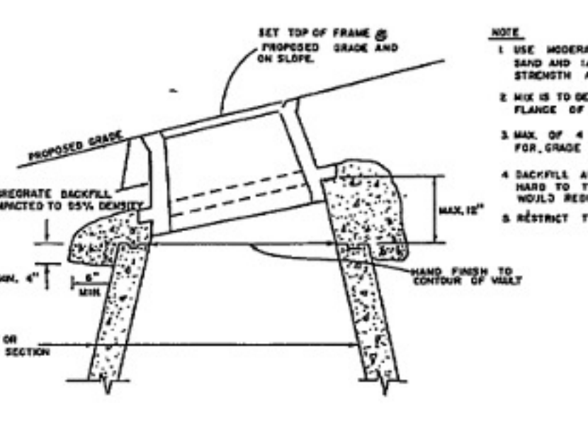
MANHOLE FRAME & COVER ADJUSTMENT
