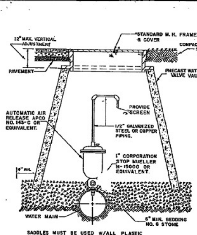
AUTOMATIC AIR RELEASE ASSEMBLY
