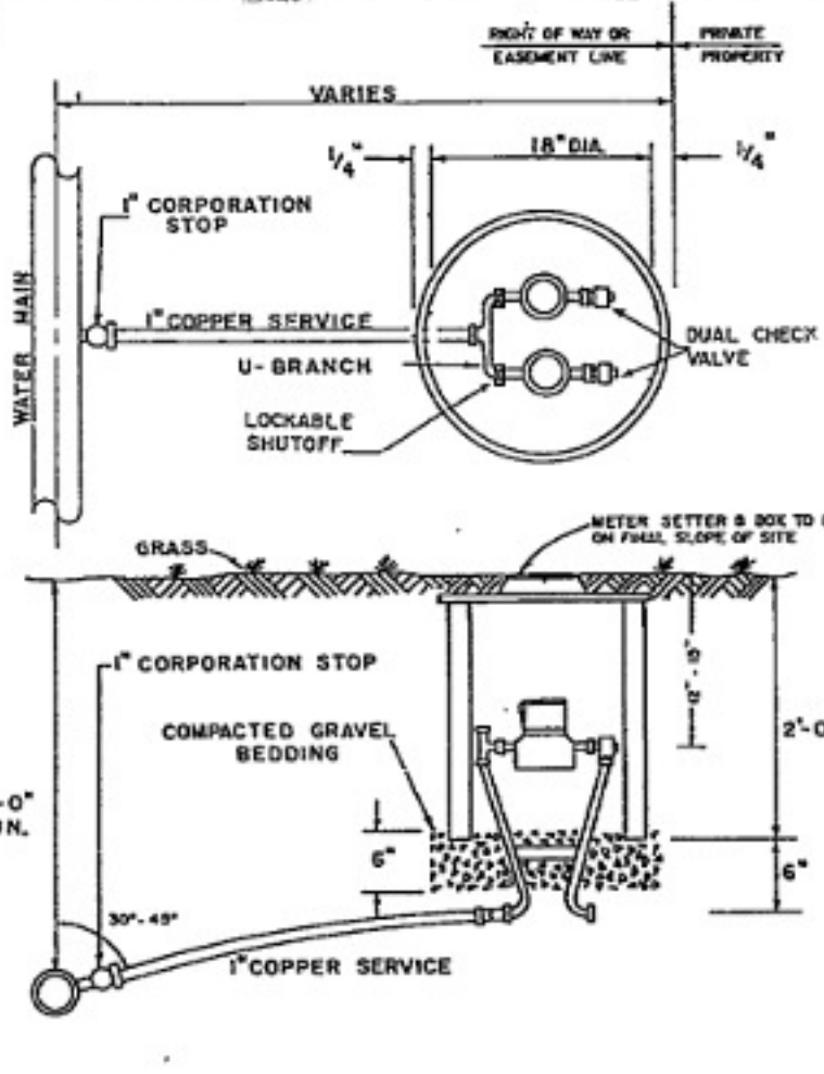
DOUBLE RESIDENTIAL WATER SERVICE
