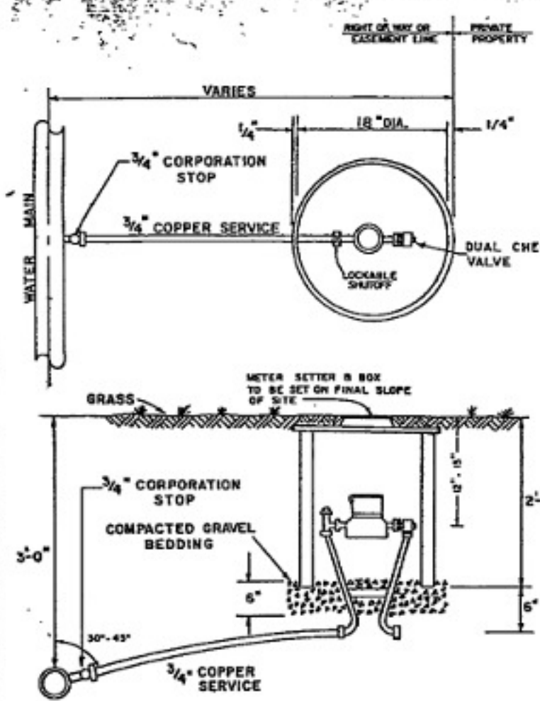
SINGLE RESIDENTIAL WATER SERVICE
