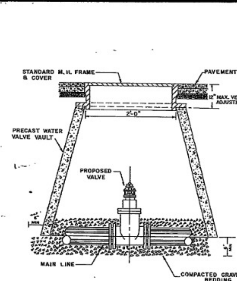
WATER LINE VALVE INSTALLATION
