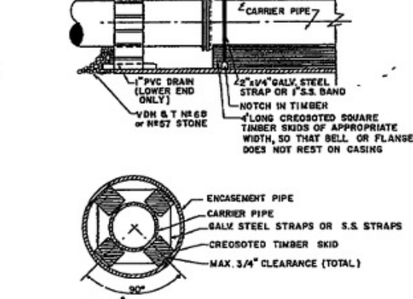
PIPE SUPPORT IN CASING PIPE
