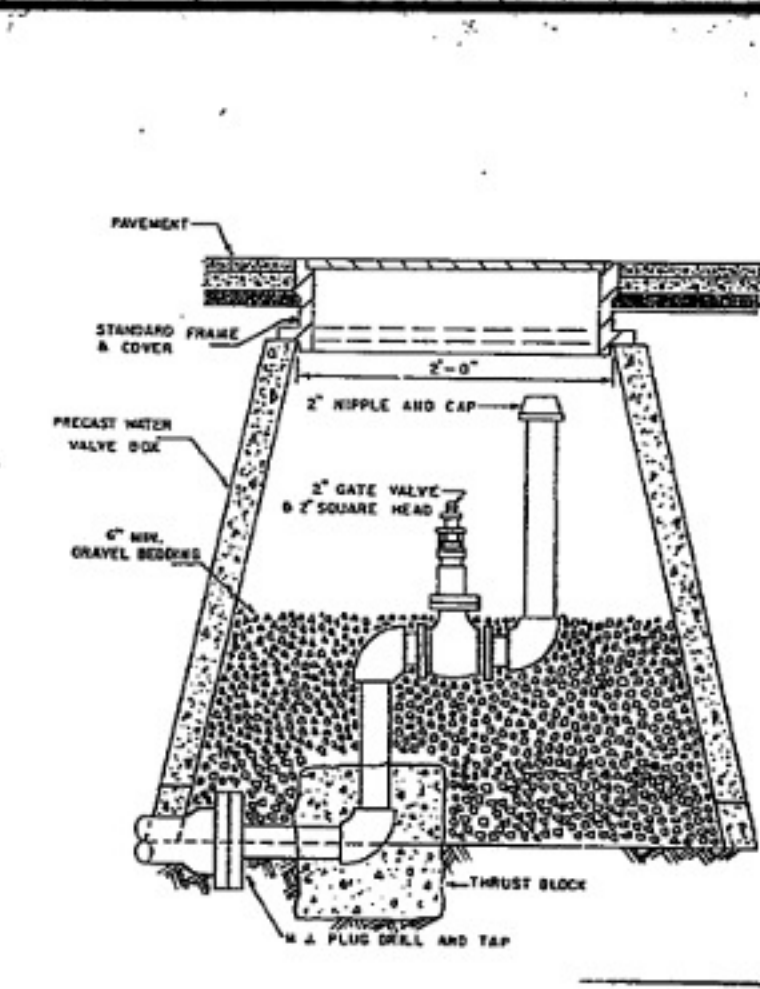
PERMANENT END OF LINE
