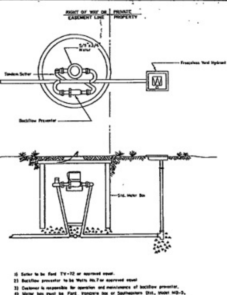
TYPICAL SPRINKLER SERVICE
