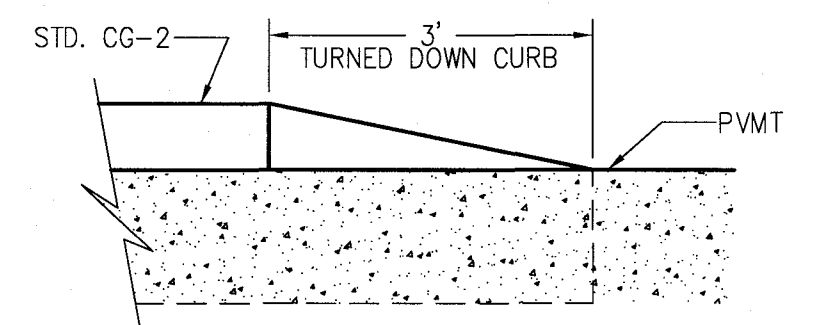
TURNED DOWN CURB DETAIL
