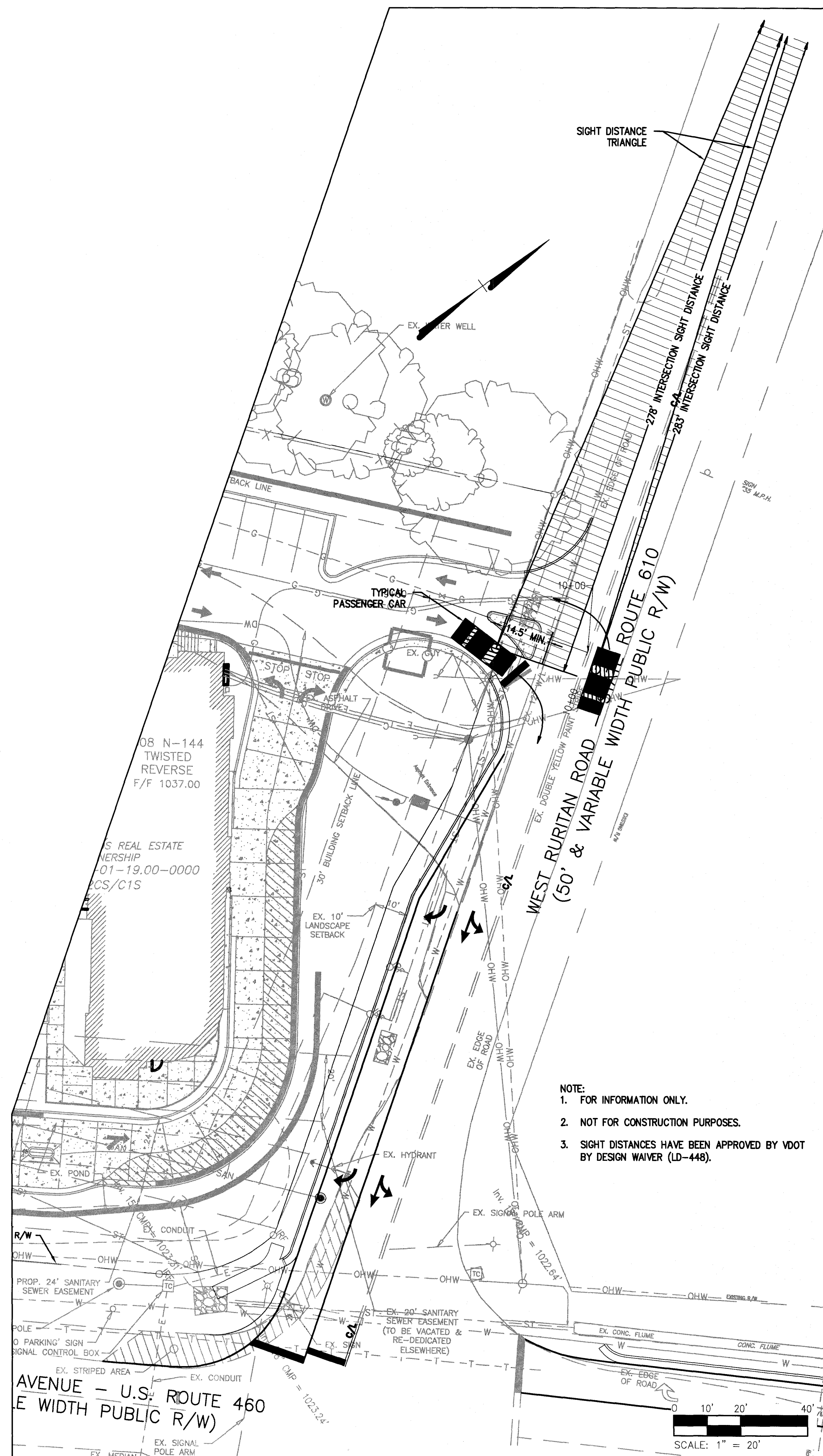
INTERSECTION SIGHT DISTANCES
