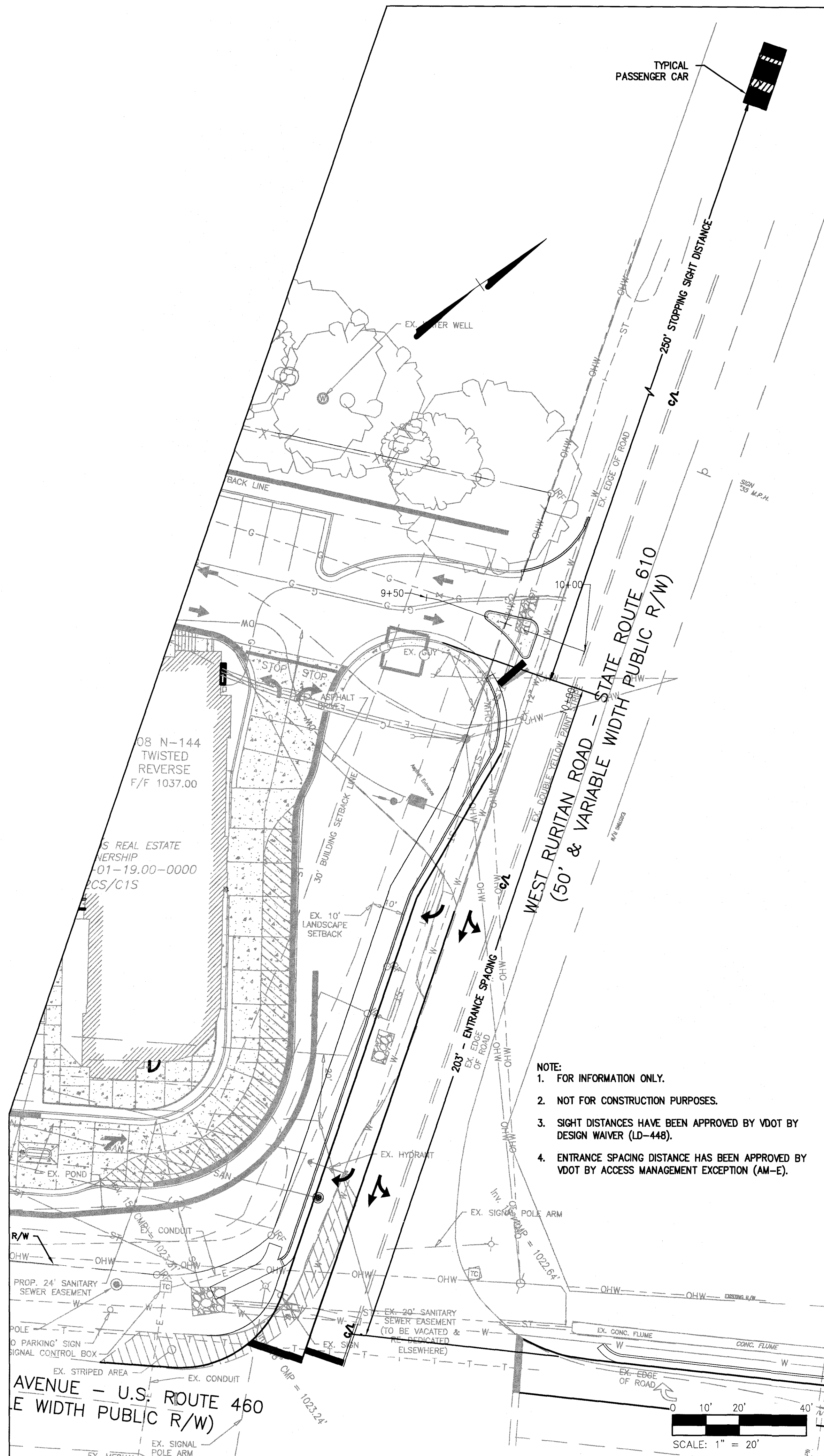
ENTRANCE SPACING AND STOPPING SIGHT DISTANCES
