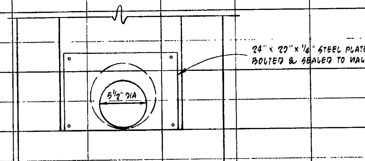
DETAIL OF RESTRICTOR PLATE IN INLET "B"
