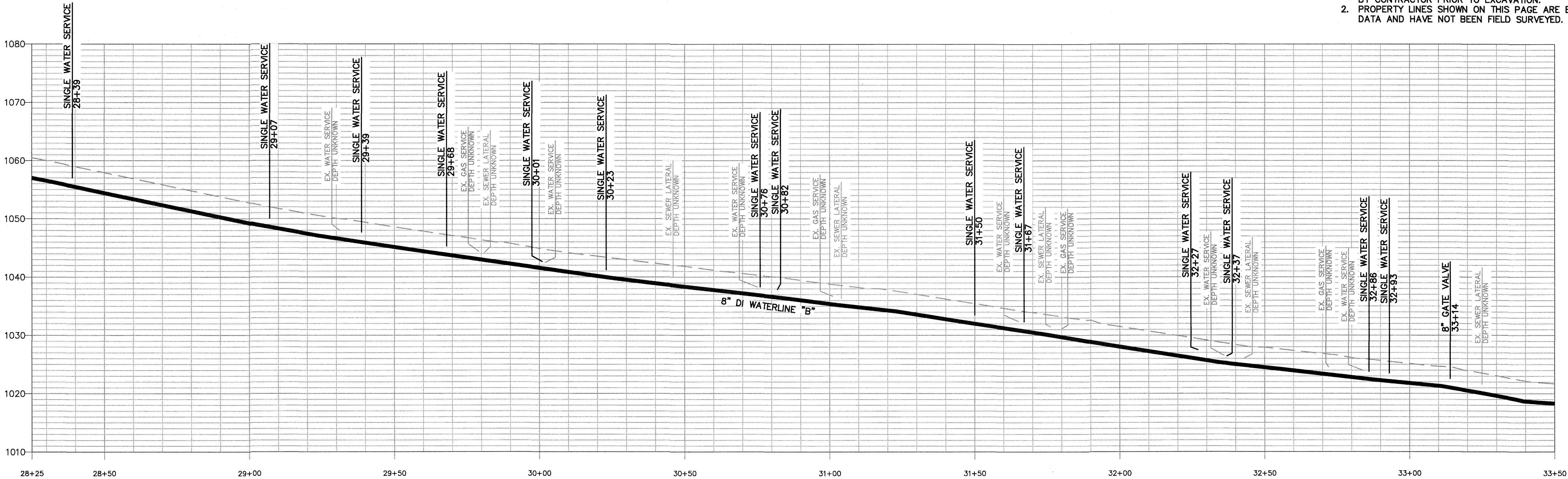
WATERLINE "B" SCALE VERTICAL: 1" = 10' HORIZONTAL: 1" = 20'
