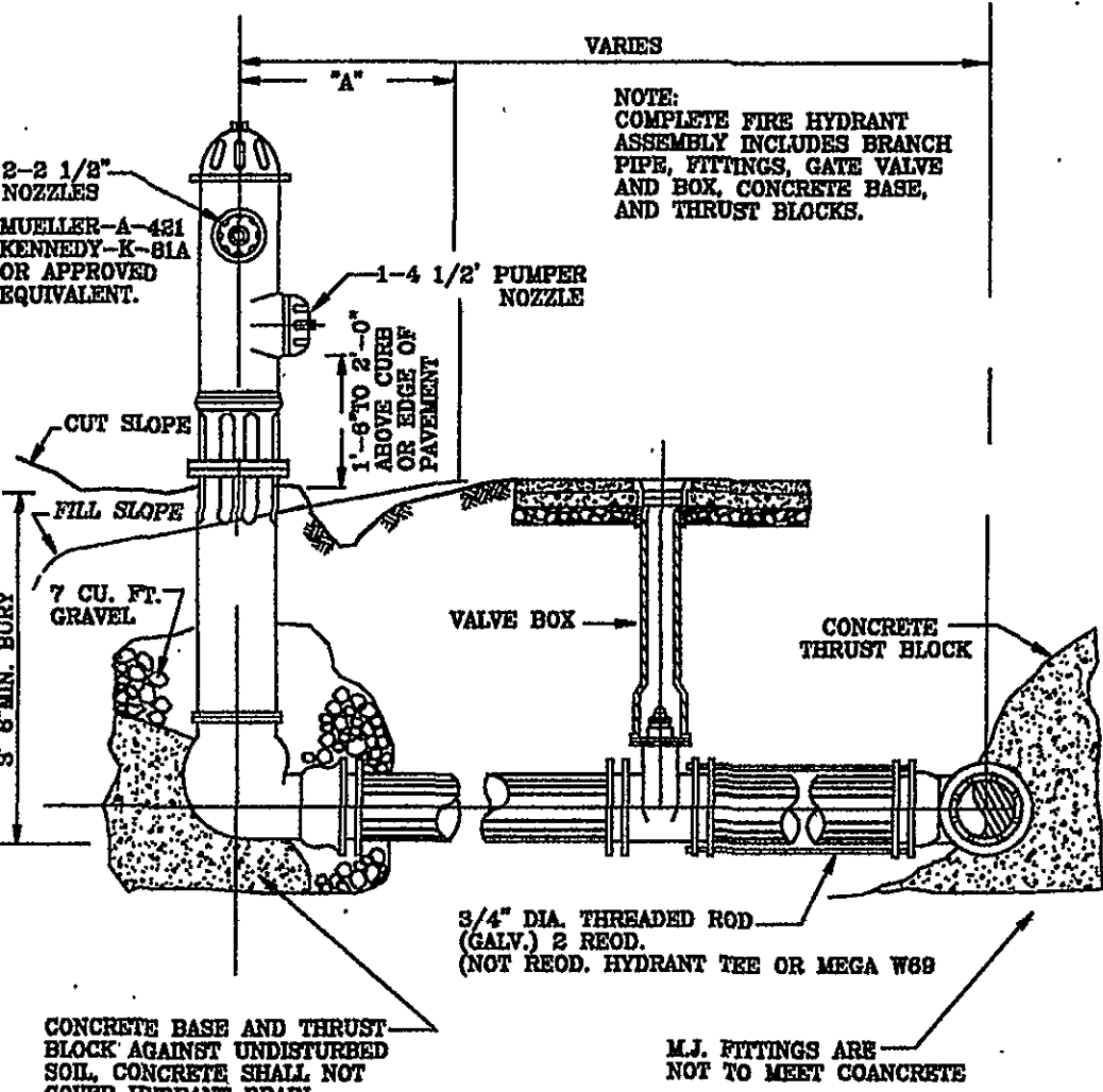
FIRE HYDRANT ASSEMBLY
