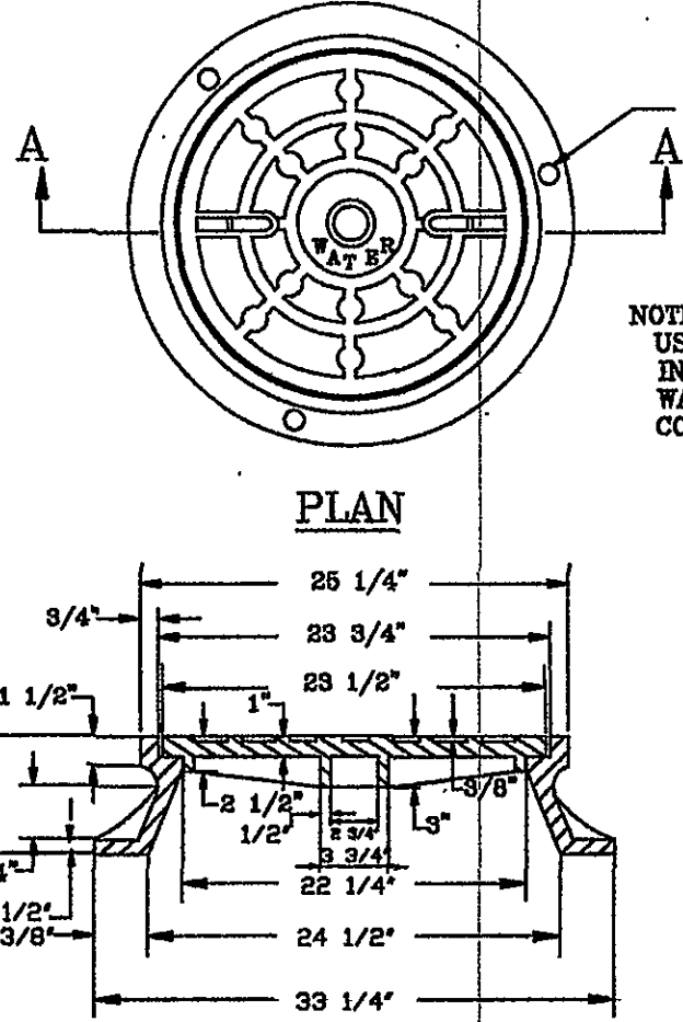
MANHOLE FRAME AND COVER
