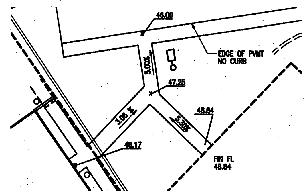
ACCESSIBLE ENTRY 5 & 6 SCALE 1"=20'
