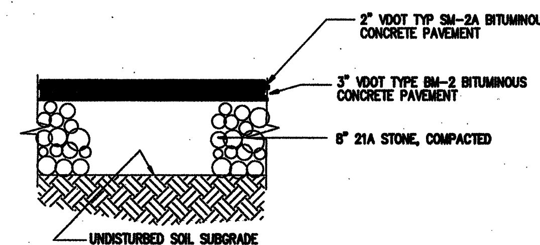
PAVEMENT DETAIL - MEDIUM DUTY NO SCALE
