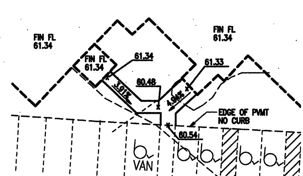
ACCESSIBLE ENTRY 1 & 2 SCALE 1"=20'
