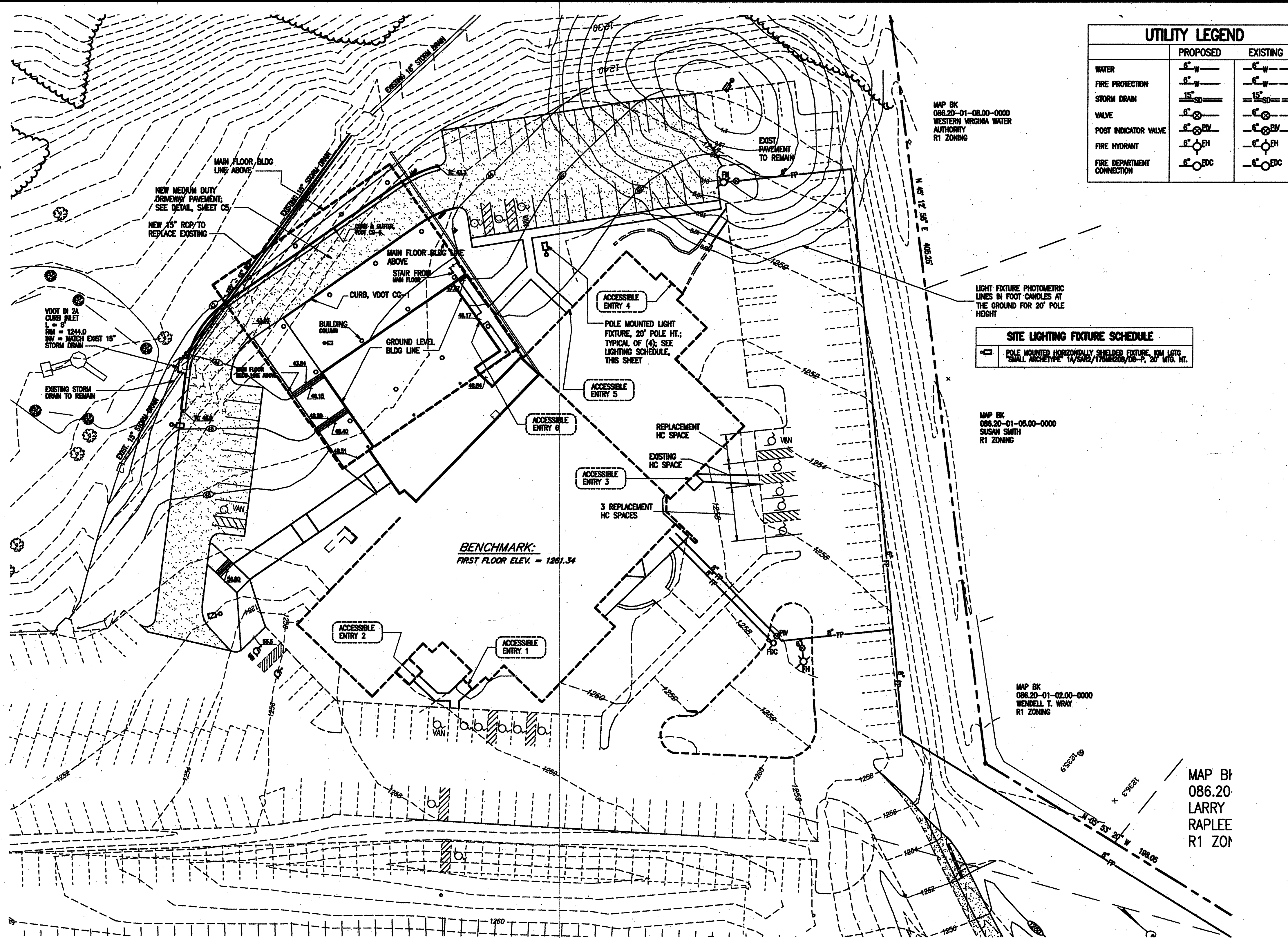
LAYOUT & GRADING PLAN - SANCTUARY ADDITION 1" = 30'
