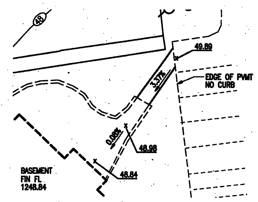
ACCESSIBLE ENTRY 4 SCALE 1"=20'
