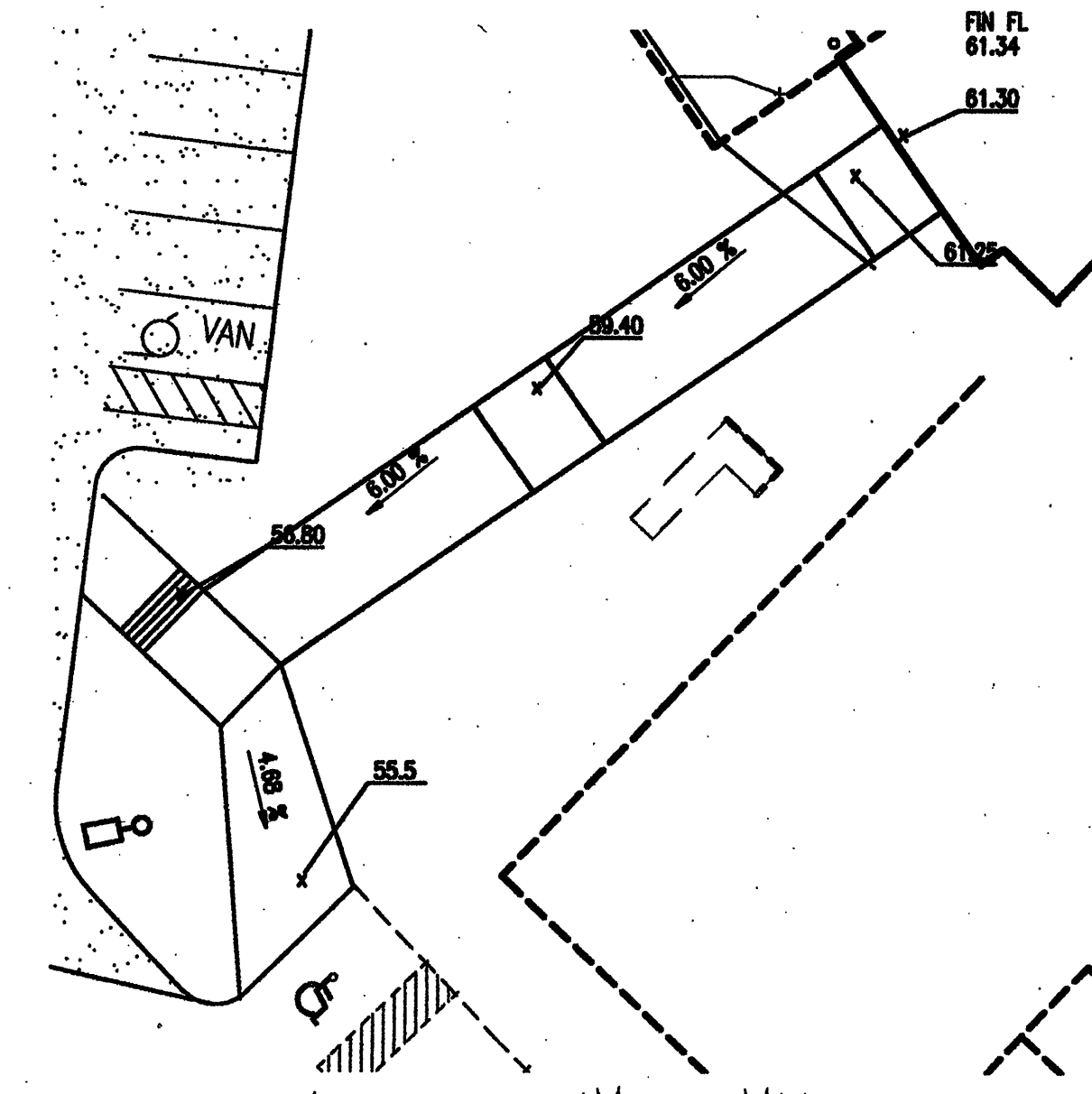
ACCESSIBLE RAMP TO MAIN FLOOR OF NEW SANCTUARY SCALE 1"=20'
