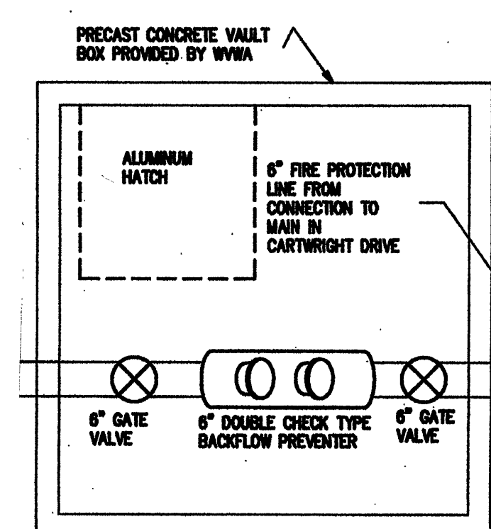
FIRE PROTECTION LINE VAULT
