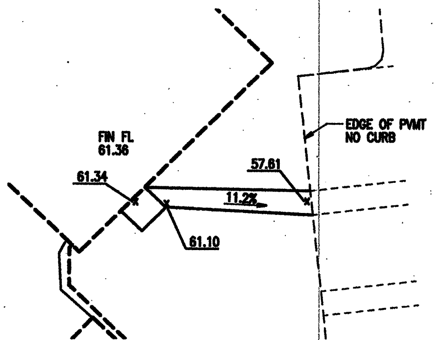
ACCESSIBLE ENTRY 3 SCALE 1"=20'
