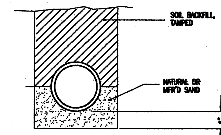
STORM & FIRE PROTECTION PIPING BEDDING DETAIL NO SCALE
