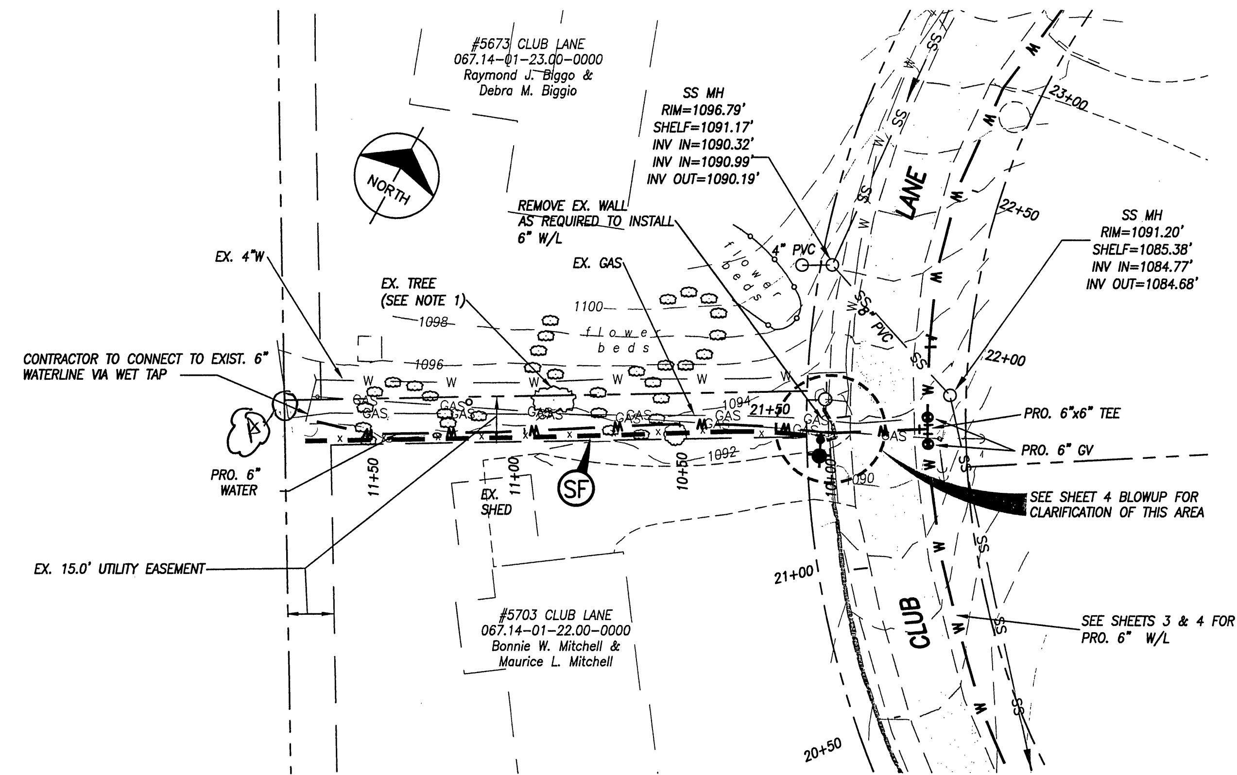
PLAN OF CLUB LANE 6" CONNECTION WATERLINE REPLACEMENT
