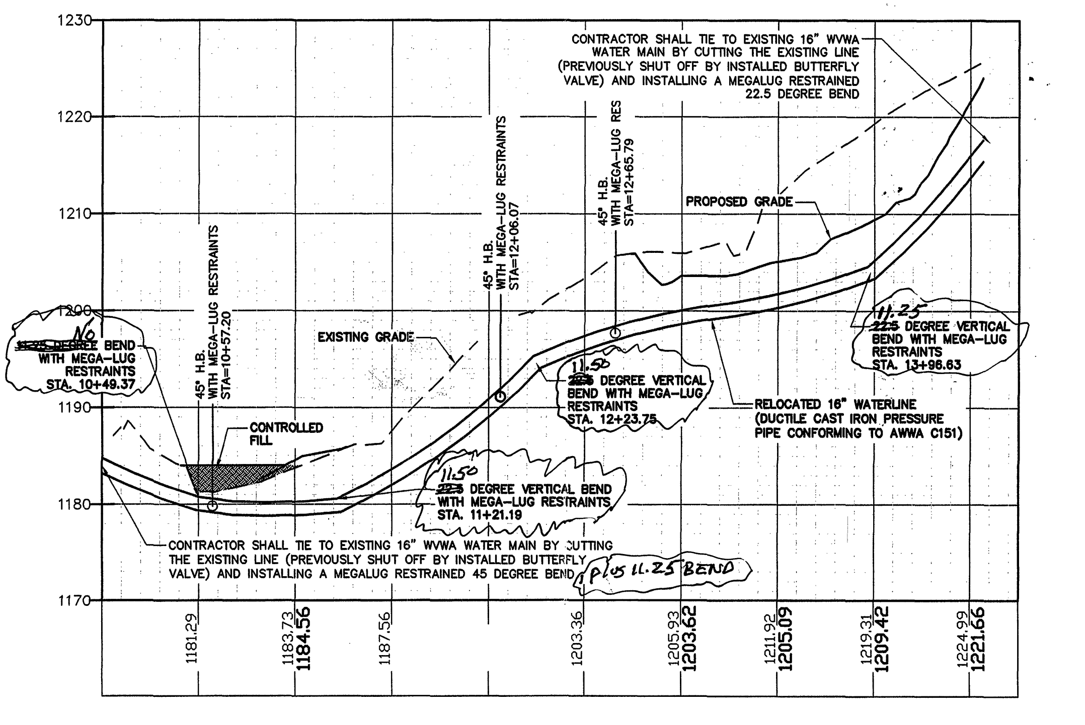
Proposed Relocation of Existing Waterline SCALE VERTICAL: 1" = 8' HORIZONTAL: 1" = 40'
